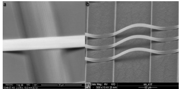
Fig. 4 SEM images of (left) flat diamond ribbon suspended across a 20 μm wide and 30 μm deep trench and (right) buckled diamond ribbons on elastomeric PDMS substrate.
