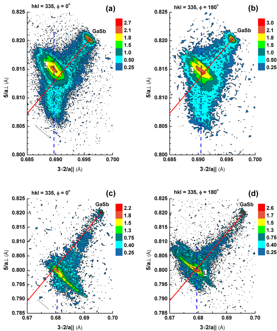
FIG. 1. Asymmetric (335) RSMs measured for structures with \text{InAs}_{0.8}\text{Sb}_{0.2} (a),(b) and \text{InAs}_{0.56}\text{Sb}_{0.44} (c),(d) in the [110] and [-1-10] directions. The reciprocal lattice point corresponding to the 1\text{-}\mu\text{m} -thick \text{InAsSb} layer is marked as L. The solid red line denotes the location of 335 reflexes of fully relaxed materials, and the vertical dashed blue line denotes that of the materials grown pseudomorphically on top of the buffer. Shown in the legend is the common logarithm of the x-ray intensity in the unit of counts/s.
