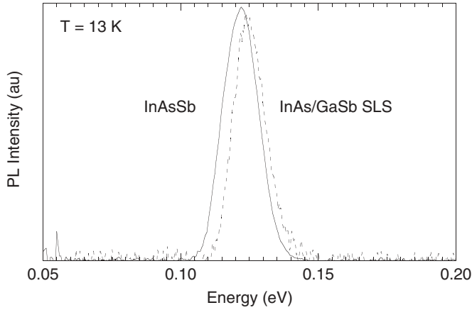
FIG. 2. PL spectra from \text{InAs}_{0.54}\text{Sb}_{0.46} grown on an \text{AlGaInSb} buffer and from a long-wave \text{InAs/GaSb} superlattices grown on a \text{GaSb} substrate, both measured at T = 13 K under the same excitation of 0.1 W. The PL was excited by a Nd:YAG cw laser with a beam diameter of 0.5 mm.
