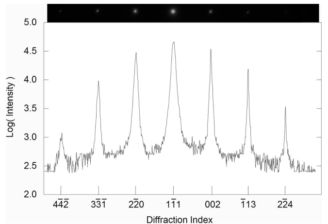
FIG. 5. TEM-SAD pattern and the intensity profile through \bar{1}\bar{1}1 (top inset) from an \text{InAs}_{0.59}\text{Sb}_{0.41} film showing no extra diffraction features that would indicate ordering. Ordering spots, if present, would appear halfway in between the major diffraction spots.
