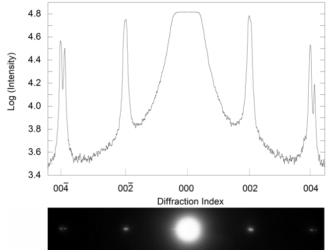
FIG. 7. TEM-SAD pattern (bottom inset) and the intensity profile along (002) from a substrate rotation-induced compositional superlattice.
