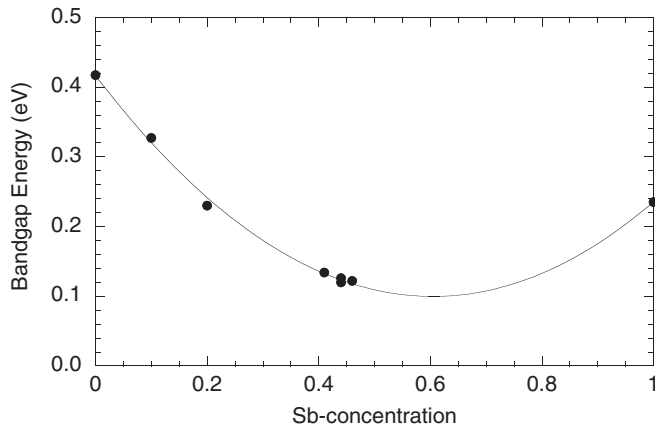
FIG. 3. Energy dependence of 13 K PL maxima on composition x in \text{InAs}_{1-x}\text{Sb}_x epitaxial layers: \text{InAs} epilayer grown on \text{InAs} substrate, \text{InAs}_{0.9}\text{Sb}_{0.1} epilayer grown nearly lattice matched to \text{GaSb} substrate, \text{InAsSb} epilayers with x = 0.20 to 0.46 grown on \text{AlGaInSb} buffers on \text{GaSb} substrates. The best fit was obtained with a bowing parameter of 0.87 eV.
