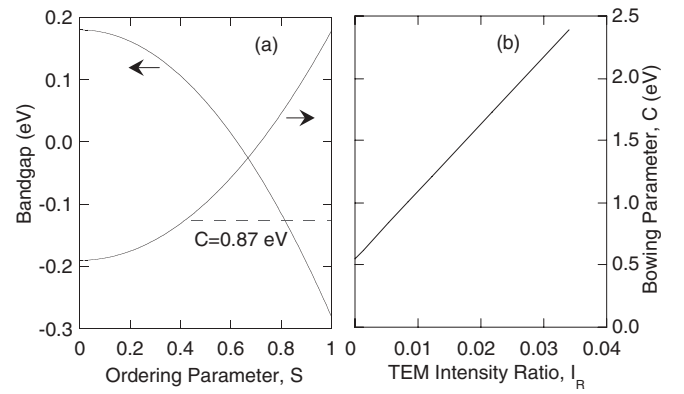
FIG. 4. The calculated relationships between (a) ordering parameter S , band gap, and bowing parameter C and (b) TEM intensity ratio I_R and bowing parameter C of \text{InAs}_{0.5}\text{Sb}_{0.5} . See text for details. The horizontal line indicates the measured bowing parameter C = 0.87 eV.
