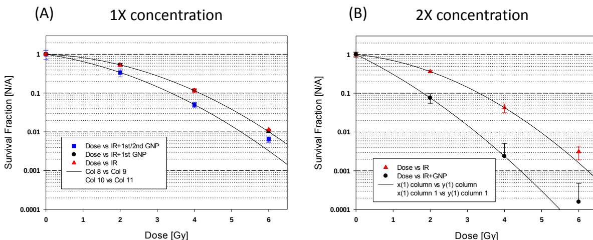
Figure 6. Survival fraction curves from clonogenic assays from the 100 nm gold nanoparticles applied on MDA-MB-231 with two different concentrations. 1X concentration: 2 \times 10^8 particles/ml. 1 st GNP in (A): Intracellular nanoparticles. 2 nd GNP in (A): extracellular nanoparticles. GNP in (B): intra- and extra-cellular nanoparticles.
