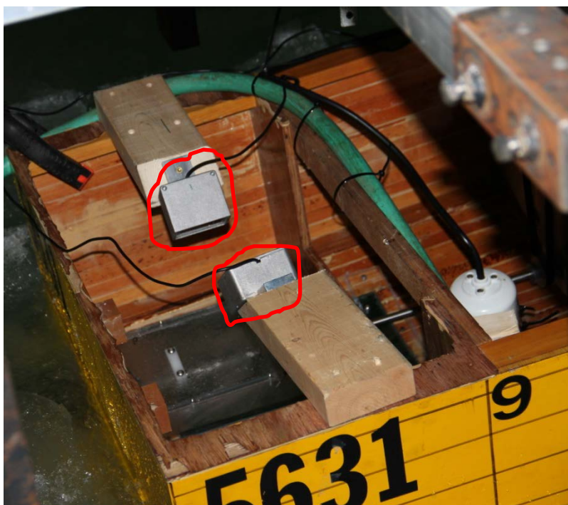
Figure 18. Above-water camera locations for waterjet intake system tests.
