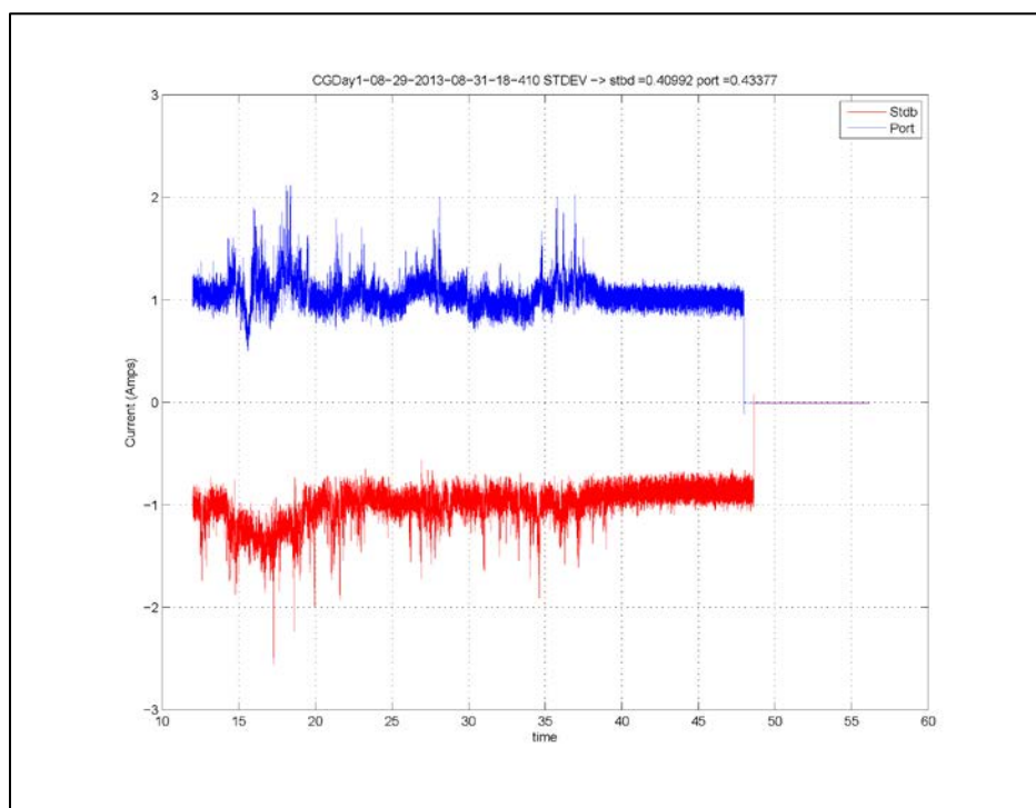
102 mm-thick ice field, carriage speed of 0.8 ms -1 Current vs. time
