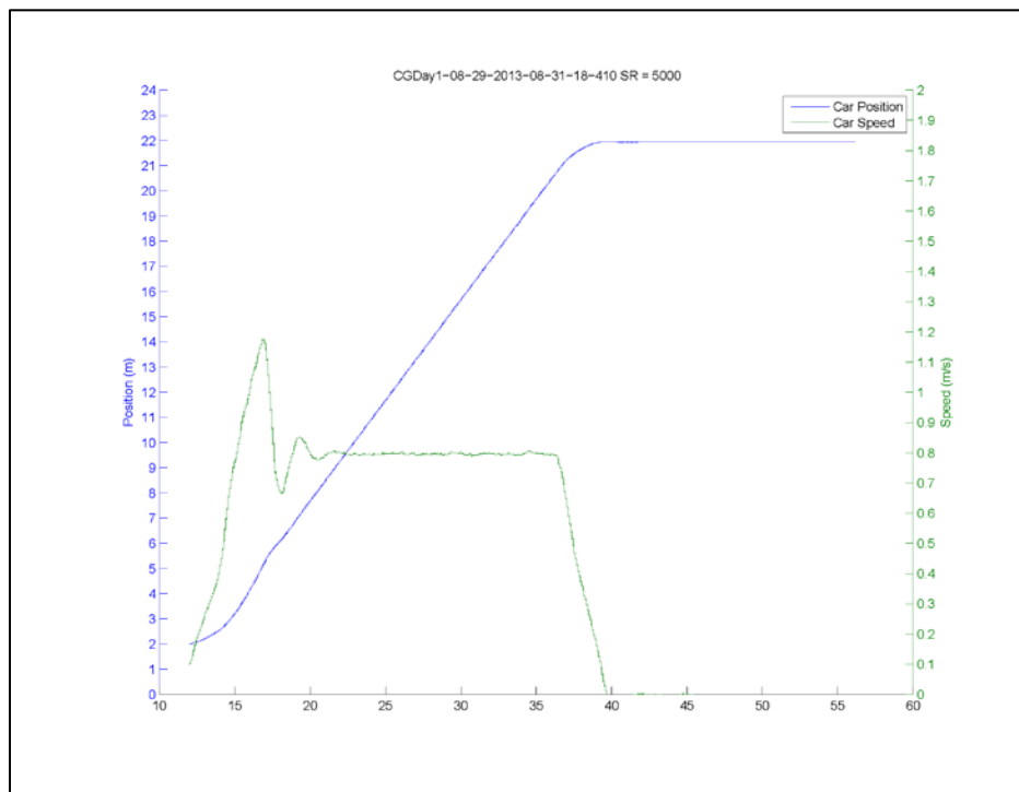
102 mm-thick ice field, carriage speed of 0.8 ms -1 Speed and position plot vs. time
