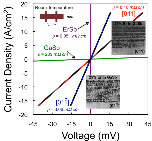
Fig. 4 Current-voltage characteristics parallel and perpendicular to embedded ErSb nanorods in GaSb. For comparison measurements for GaSb and ErSb epitaxial layers are also shown.
