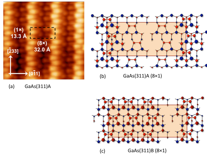
Fig. 6 (a) STM image of GaAs(311)A (8×1) surface reconstruction and predicted atomic models for (b) GaAs(311)A and GaAs(311)B. The red atoms correspond to As and the blue Ga. Both surfaces satisfy electron counting.
