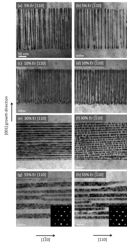
Fig. 2 Bright field TEM images along the [110] and [-110] zone axes of (a,b) a 250 nm \text{Ga}_{0.95}\text{Er}_{0.05}\text{Sb} (001) layer grown at 500^\circ\text{C} . The ErSb phase segregates from the GaSb and forms nanorods aligned along the surface normal. (c,d) TEM images of a \text{Ga}_{0.9}\text{Er}_{0.1}\text{Sb} (001) nanocomposite showing a higher density of vertical nanorods. (e,f) TEM images of a \text{Ga}_{0.7}\text{Er}_{0.3}\text{Sb} (001) nanocomposite. At 30% Er, the ErSb nanorods switch direction and lie in-plane along the [-110] (g,h) TEM images of a \text{Ga}_{0.45}\text{Er}_{0.55}\text{Sb} (001) nanocomposite, forming ErSb nanosheets. (inset) Electron diffraction patterns showing that the nanocomposites are single crystalline.
