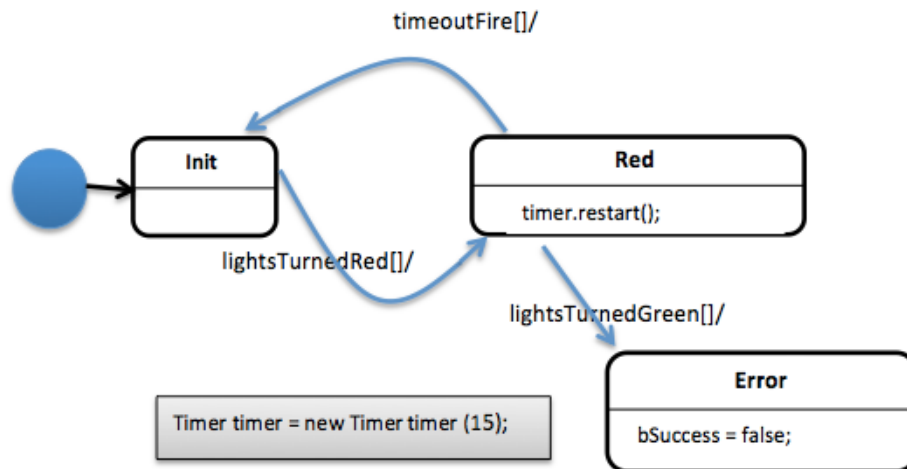
Figure 1. A statechart assertions for TLC requirement R3.
