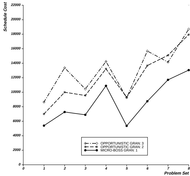
Figure 5-17: Comparison of the cost of the schedules produced by MICRO-BOSS and two coarser opportunistic schedulers under 8 different scheduling conditions.
