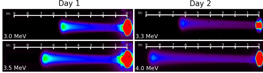
Figure 4: Four representative false-color images of the UMass - Lowell proton beam experiments. The images on the left were taken on the first day of operation and have energies of 3.0 MeV and 3.5 MeV, respectively. Day 2 images on the right have 3.3 MeV and 4.0 MeV, respectively. The images from Day 2 appear “dimmer” due to color-scaling and different beam currents.
