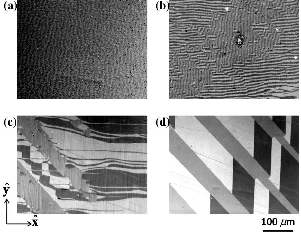
Figure 3.17: Domain structure of 17S as a function of silica gel polishing time (a) t = 0 , (b) t = 20 min, (c) t = 50 min, (d) 75 min.
