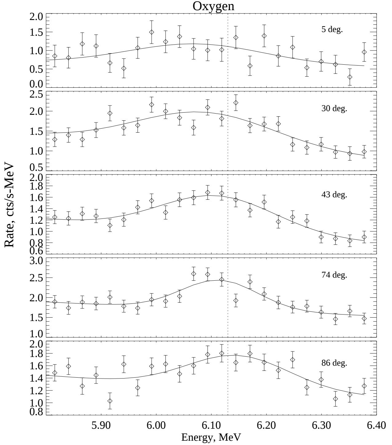
Fig. 4.— Gaussian line fits to the ^{16}\text{O} de-excitation line observed in flare spectra at different heliocentric angles. The dotted line shows the rest energy of the de-excitation.
