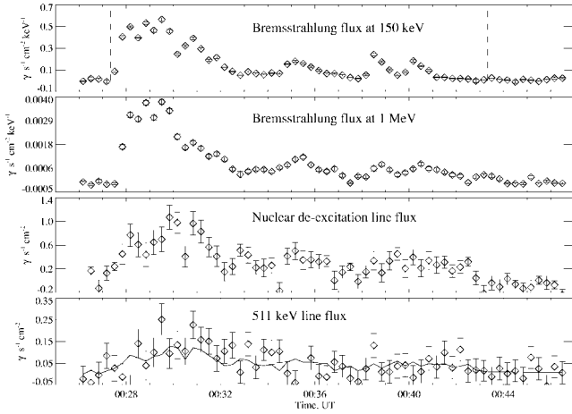
FIG. 1.—Time histories of the solar bremsstrahlung, nuclear de-excitation lines, and 511 keV annihilation line during the 2002 July 23 flare observed by RHESSI at 20 s resolution. The dashed lines indicate the time interval from 00:27:20 to 00:43:20 UT used for spectral studies. The solid curve shows the calculated annihilation line profile (see text).
