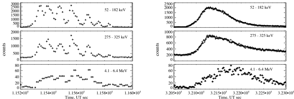
Figure 4. Comparison of flare time histories in three energy bands. Left panel, entire 1980 June 7 impulsive flare; right panel, one peak in the 1988 Dec. 16 flare.
