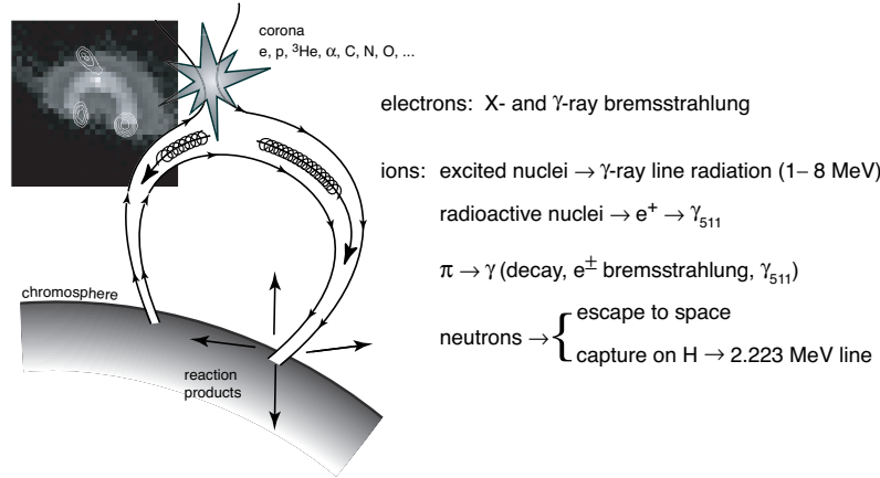
Figure 1. Schematic showing particle acceleration, transport, and interaction products during solar flares
