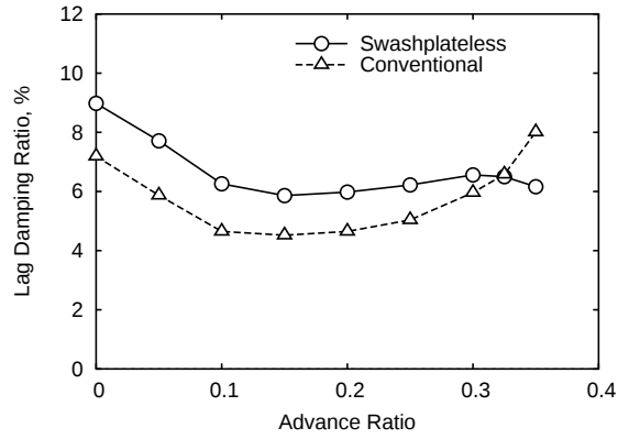
(a) Blade lag damping
