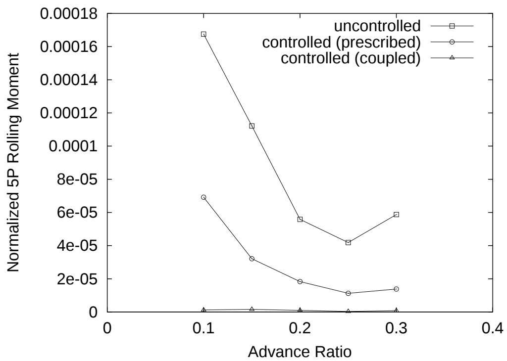
Figure 3.48: 5/rev hub rolling moment
