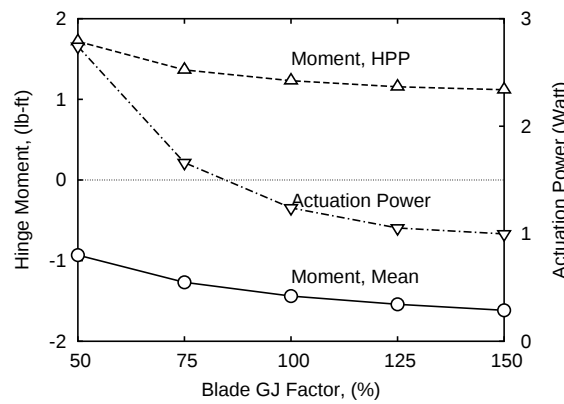
(c) Flap hinge moment and actuation power
