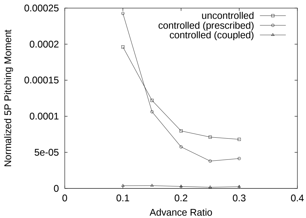
Figure 3.49: 5/rev hub pitching moment
