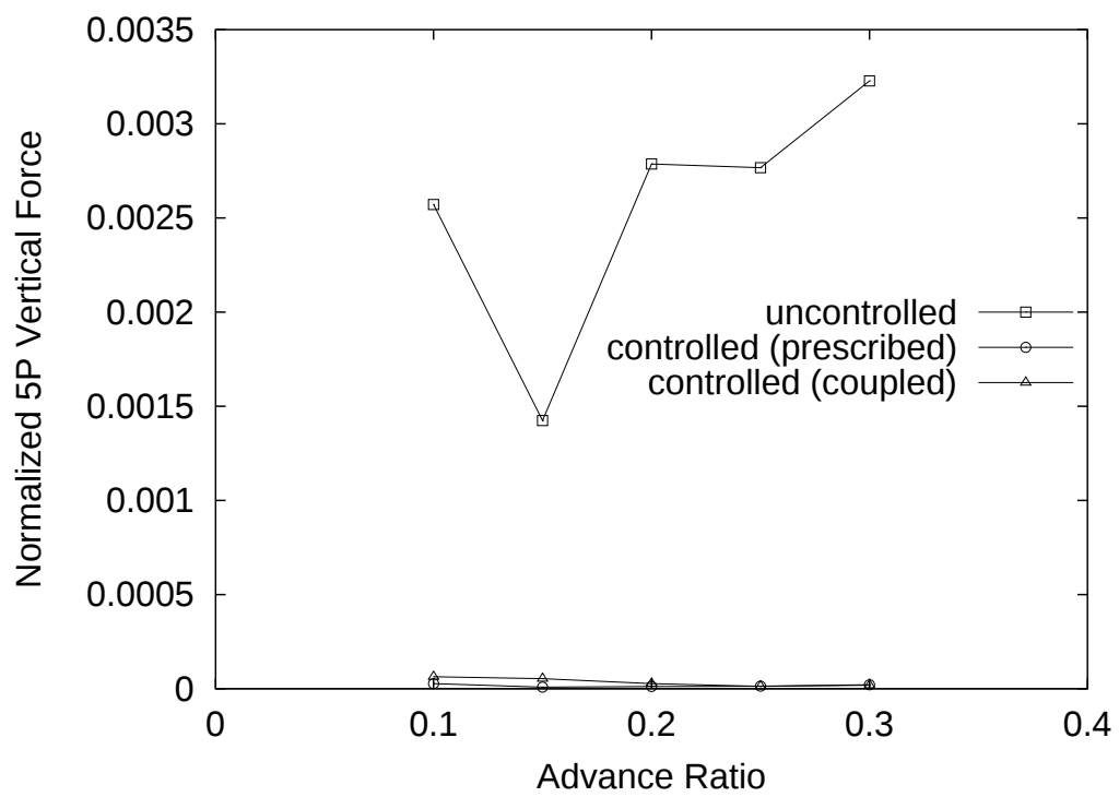
Figure 3.47: 5/rev hub vertical force
