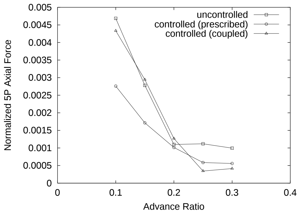
Figure 3.45: 5/rev hub axial force
