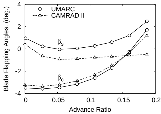
(c) Blade flapping angles
