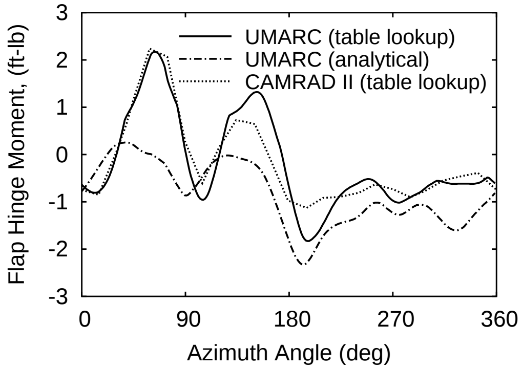
Figure 3.32: Comparison of flap hinge moment predictions of UMARC and CAMRAD II with prescribed flap motion \delta_f = 2^\circ \cos(4\psi - 240^\circ) , \mu = 0.2 , C_T/\sigma = 0.0774 , c_b/c_f = 0.29 , c_{cg}/c_f = 0
