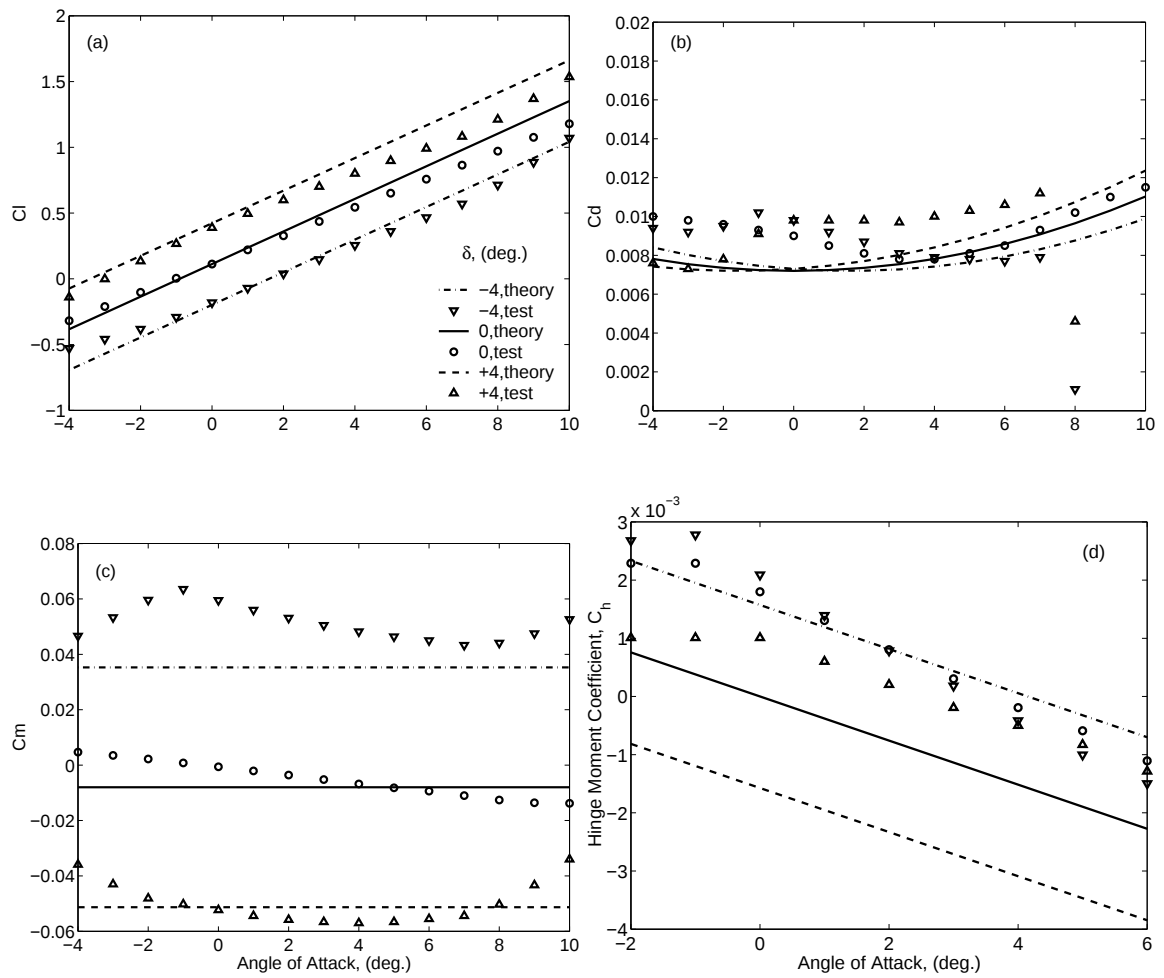
Figure 3.28: Measured and predicted aerodynamic coefficients of 2D HH-10 airfoil with 0.35 plain trailing-edge flap (10%c overhang, Mach = 0.45); (a) lift (b) drag (c) pitching moment and (d) hinge moment
