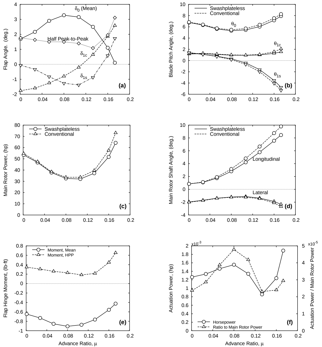
Figure 3.81: Comparisons of conventional and swashplateless rotor at different forward speeds with pitch index angle of 18^\circ
