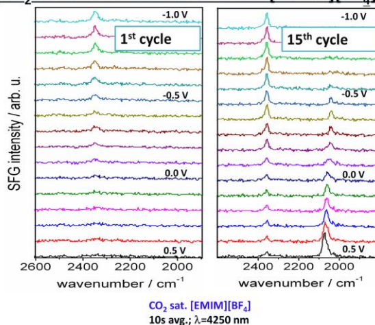
Fig. 17. \text{CO}_2 reduction to \text{CO} with low overpotential is a critical step in economic production of syngas \text{CO} + \text{H}_2 . An ionic liquid electrolyte \text{EMIM-BF}_4 substantially lowers the barrier to \text{CO}_2 reduction by stabilizing the intermediate \text{CO}_2^- . These SFG spectra show \text{CO}_2 adsorbed on a Pt electrode disappear while \text{CO} builds up, in a spectroelectrochemical cell.
