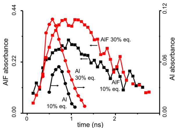
Fig. 10. Time resolved absorption intensities for Al and AlF in flash-heated Al/Teflon. The AlF absorption has a two-part rise with the faster part from AlF created in the condensed phase and the slower part from AlF created in an expanding gas cloud.
