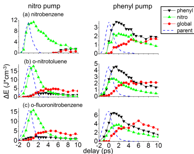
Fig. 3. IR-Raman data on nitrobenzenes. In the left column, IR pulses were used that pumped energy into the nitro groups. In the right column the phenyl groups were pumped by pulses with about the same frequency. In nitrobenzene, almost no energy flows from nitro to phenyl but some energy flows from phenyl to nitro. An ortho substituent such as methyl or fluorine turns on the nitro-to-phenyl channel.
