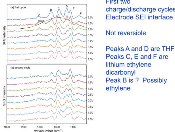
Fig. 18. SFG studies of the formation of a solid-electrolyte interphase (SEI) layer on an anode during lithium-ion battery chemistry during two successive cycles of charging and discharging.
