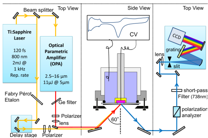
Fig. 16. Block diagram of laser apparatus for spectroelectrochemistry. The nonlinear coherent vibrational spectroscopy method termed “vibrational sum-frequency generation” (SFG) selectively detects molecules at the electrode-electrolyte interface, ignoring species in the bulk electrolyte.
