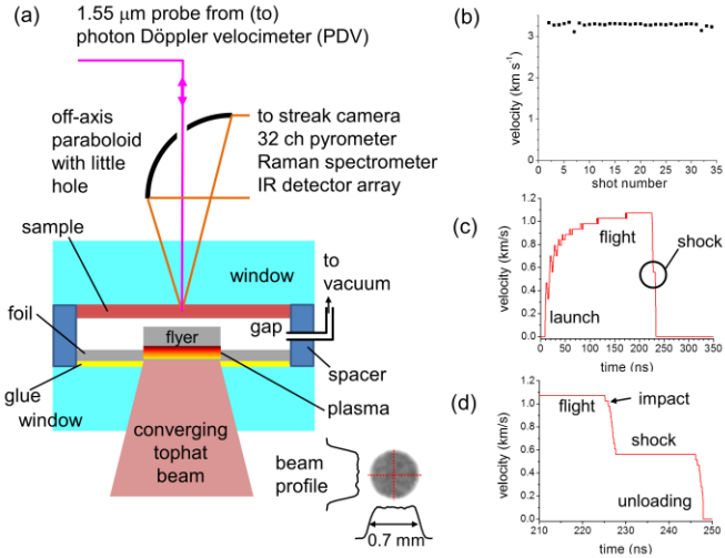
Fig. 11. Schematic of laser apparatus for spectroscopy of materials shocked by a laser-launched Al flyer. Notice uniform 0.7 mm laser beam profile generated by a diffractive optic. (a) Sample and light collection. (b) Speeds of 33 flyer launches were remarkably reproducible. (c) Doppler velocimeter history of a flyer launched at 1 km/s. (d) Time-expanded velocity history showing 15 ns duration constant shock in a glass target.
