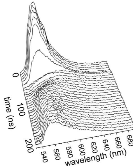
Fig. 12. Time-resolved emission from R6G dye in PMMA polymer during a 1 km/s impact. When the shock front arrives, the dye emission loses intensity and redshifts. A computer extracts the time-dependent redshift.
