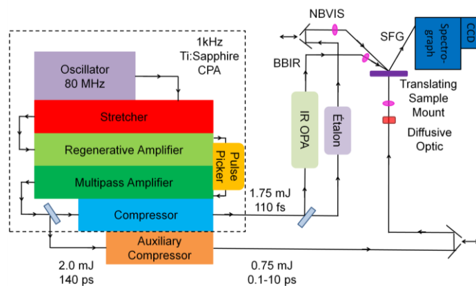
Fig. 4. Block diagram of laser apparatus used for ultrafast T-jump or shock compression. The flash-heated or shocked molecular monolayers are probed using nonlinear coherent vibrational spectroscopy.
