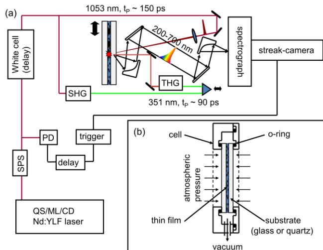
Fig. 9. Schematic of picosecond laser apparatus to study the time-resolved optical emission and absorption from Al/Teflon reactive materials.
