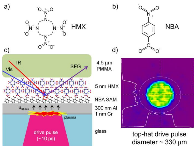
Fig. 5. Sample construction for ultrafast shock vibrational spectroscopy. A monolayer of NBA is deposited onto a metal film. The nitro groups are probed by nonlinear coherent vibrational spectroscopy. A layer of \delta -HMX a few molecules thick can be grown on top of the NBA. A diffusive optic is used to produce a spatially-uniform drive beam.
