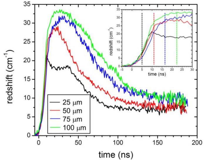
Fig. 13. Time-resolved emission redshift from R6G dye in PMMA during 1 km/s shocks from different thickness flyer plates. The mechanical response of the PMMA is highly dependent on the shock duration.
