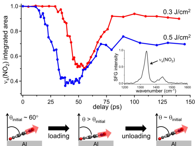
Fig. 6. Ultrafast shock vibrational spectroscopy of nitrobenzoic acid monolayer with shocks in the 1 GPa range. The shock causes the molecules to tilt, which reduces the nitro group signal. The effect started sooner when the laser fluence was 0.5\text{ J/cm}^2 because the shock traveled faster.
