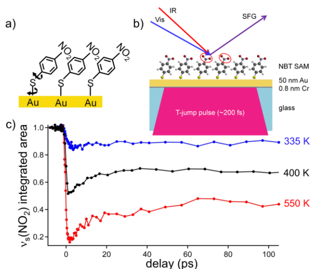
Fig. 8. Ultrafast flash-heating of nitrobenzenethiol monolayer probed by nonlinear coherent spectroscopy of the nitro group. A femtosecond white light pulse is used to monitor the temperature of the gold substrate. After \sim 10 \text{ ps} , the gold and the monolayer are in equilibrium and the T-jump can be as large as 250K.
