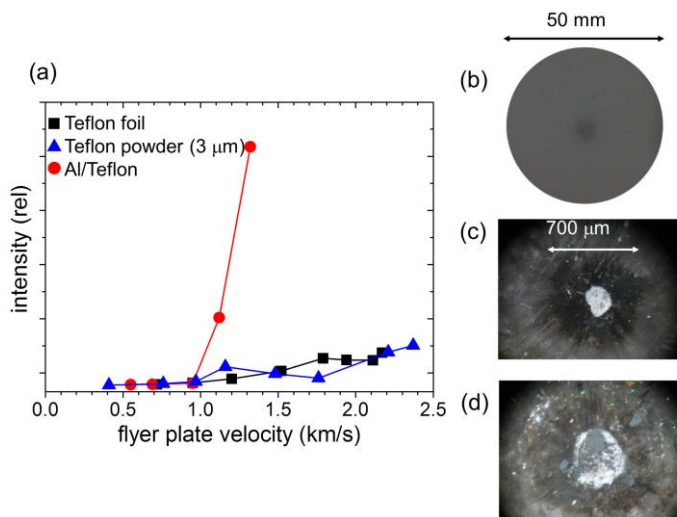
Fig. 14. (a) Emission intensity from Al (50 nm)/Teflon (3 \mu\text{m} ) RM impacted at different velocities. There is an initiation threshold at about 1 km/s. (b) Photo of Al/Teflon uniform film on optical window. (c) Photo after impact by 700 \mu\text{m} Al flyer, of Teflon only. (d) Photo after impact of reactive Al/Teflon showing vaporized region.
