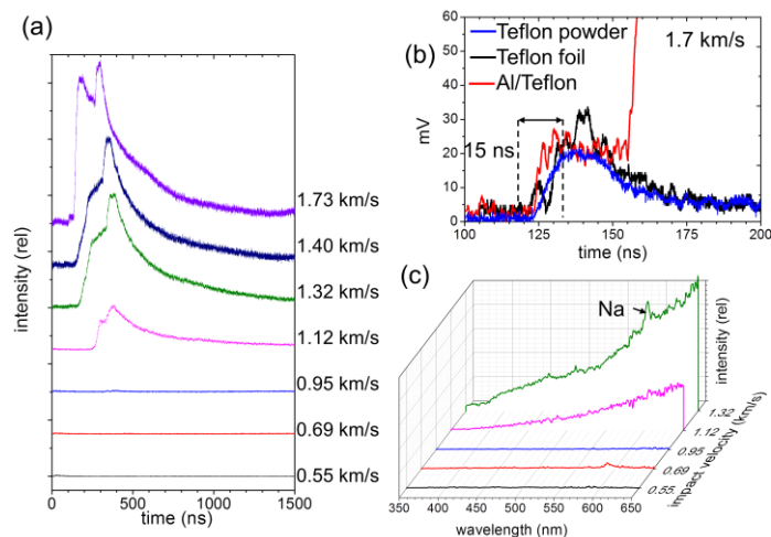
Fig. 15. (a) Emission intensity transients from Al/Teflon impacted by Al flyer plates at different speeds. (b) Al/Teflon emission with 1.7 km/s impact looks like Teflon alone until after the shock unloads, when it increases dramatically, indicating initiation. (c) Emission spectra near impact velocity threshold.
