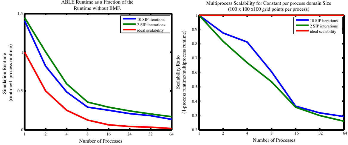
Figure 3. Scalability results for the red-black SIP-based SIMPLE integration scheme. (a) Normalized ABL runtime compared with ideal scalability by dividing a constant-size domain over an increasing number of processes. (b) Scalability based on keeping the number of grid points per process constant. Adding processes, requires increasing the total computational domain size. All runtimes are normalized by the original serial version of ABL without the overhead associated with including BMF.
