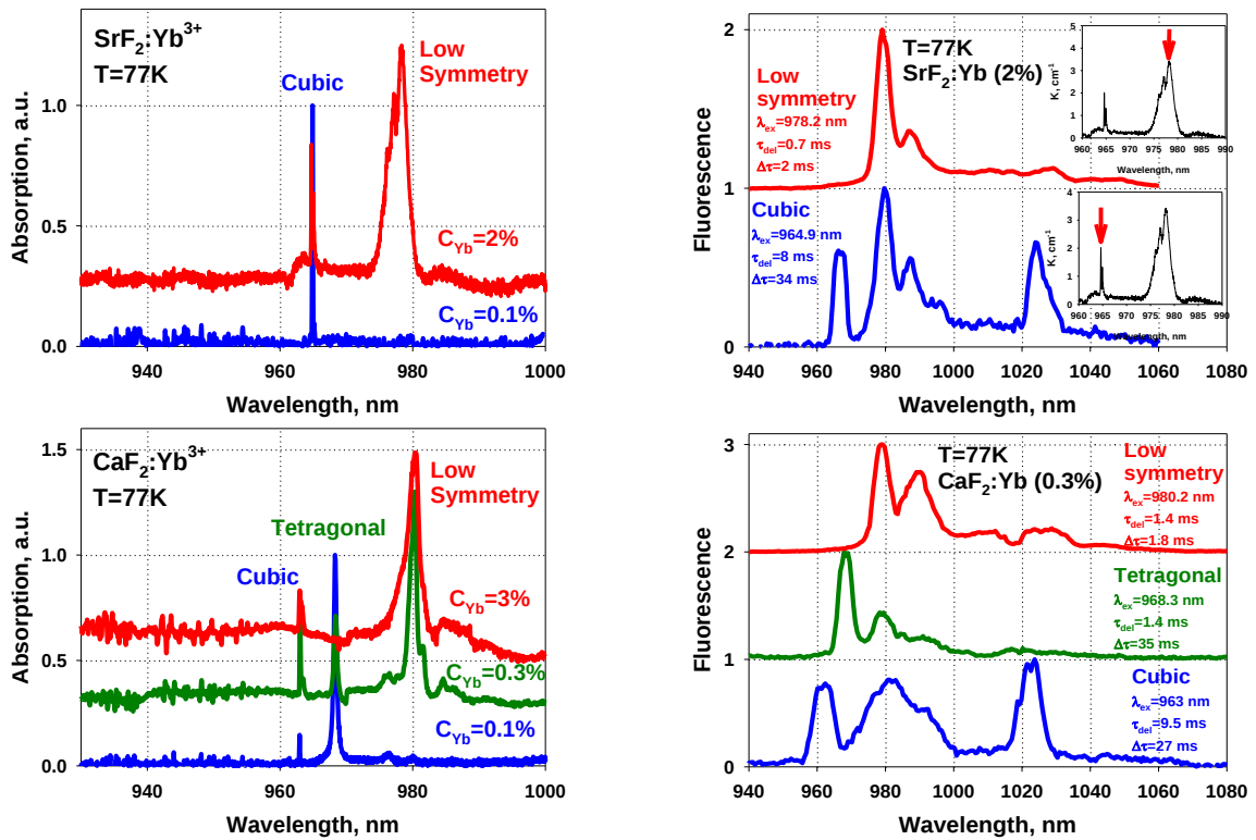
Fig.10 Absorption and fluorescence (time and spectrally resolved) spectra of different types of optical centers in SrF 2 and CaF 2 crystals.
