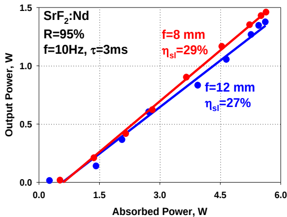
Fig.40 Optimization of the pump mode to cavity mode for the \text{SrF}_2:\text{Nd}^{3+} single crystal.
