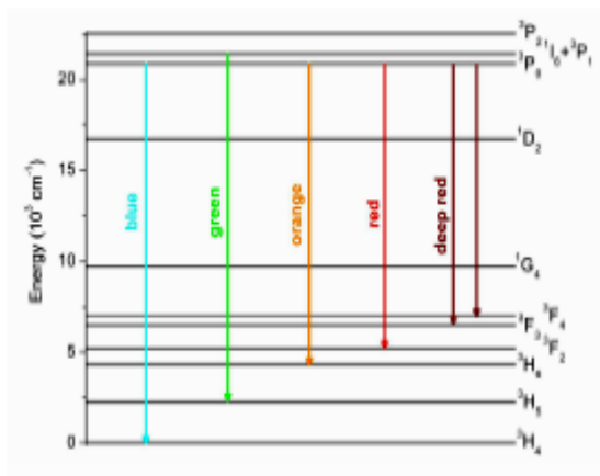
Fig.43 \text{Pr}^{3+} ion fluorescence channels in the visible spectral range
