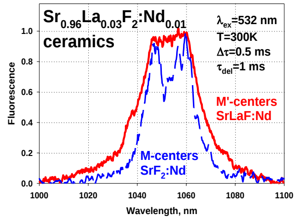
Fig.31 Fluorescence spectra of Nd-La and Nd-Nd paired centers in SrF 2 -LaF 3 and SrF 2 ceramics.
