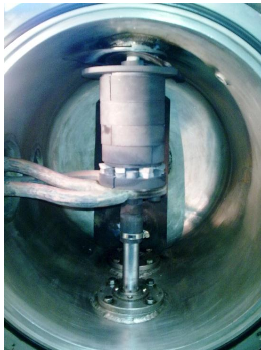
Fig.2 Modified chamber for hot formation of fluoride ceramics from single crystals.
