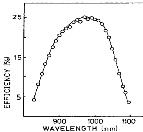
Fig.46 Tuning curve of \text{LiF:F}_2^+ color center laser.
