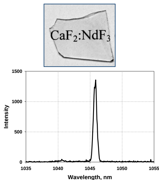
Fig.42 Oscillation spectrum of \text{CaF}_2:\text{Nd}^{3+} ceramics under laser diode pumping.
