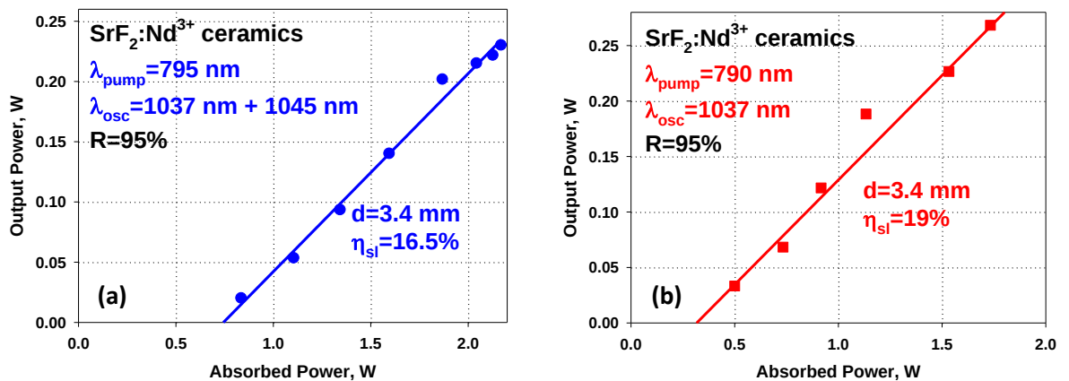
Fig.33 Output power versus pump power characteristics of \text{SrF}_2:\text{Nd}^{3+} ceramics for laser diode pumping into the absorption maximum of: (a) 795 nm for excitation of both L- and M-centers and (b) 790 nm for excitation of mostly \text{Nd}^{3+} L-centers.
