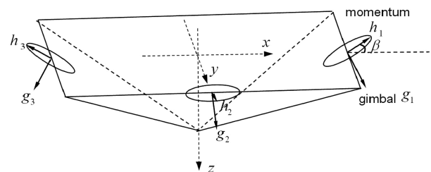
Fig. 6 CMG array configuration of the BRMS simulator.
