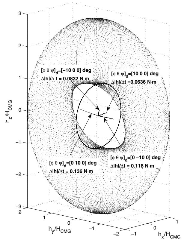
Fig. 9 Momentum trajectories and gravitational disturbances after center of gravity compensation.
