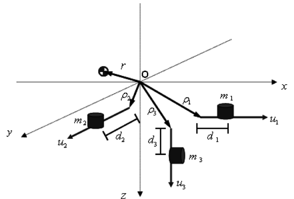
Fig. 1 Automatic mass balancing system.
