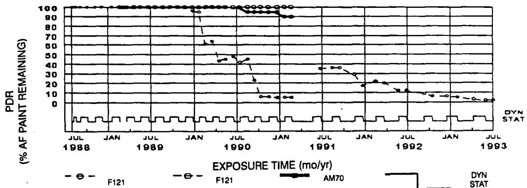
Graph B-34. Comparison of AM70 and F121 fouling rate, Cu leaching rate, and AF paint deterioration rate (PDR) in dynamic/static tests from July 1988 to July 1993.
