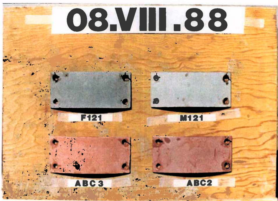
Figure 4. F121, M121 (modified F121), ABC3, and ABC2 before exposure.
