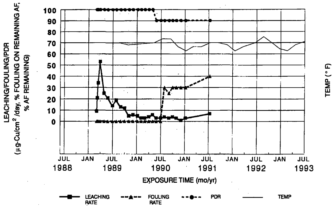
Graph B-35. Static exposure tests for Ameron 70 from July 1988 to July 1993.
