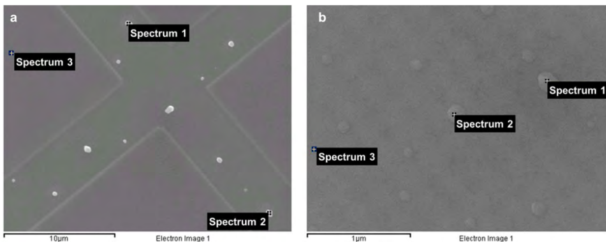
Figure 7 – Example SEM images indicating the locations of the cryo-FIB milled sample analyzed by EDS. The EDS analysis was carried out with the sample at room temperature. (a) Lower magnification image showing the large, tall features. (b) Higher magnification image showing the smaller nanodot features present in the milled region (marked as Spectra 1 and 2) and the milled floor (marked as Spectrum 3).
