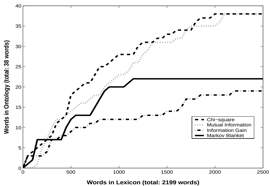
Figure 5: The four feature selection methods for the nat - gas category.
