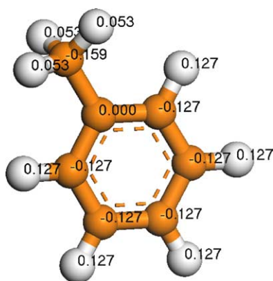
Fig. 6. Geometrically optimized structure of a toluene molecule and the corresponding atomic charges.
