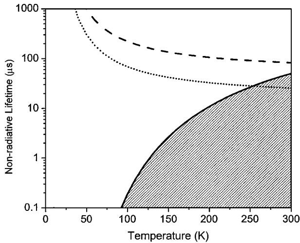
FIG. 2. Analysis of laser cooling for a 1.0 \mu\text{m} GaAs layer as a function of temperature. The solid curve is the calculated minimum nonradiative lifetime ( 1/A ) to achieve net cooling using Eq. (2) with \tau_0=500 ns and \eta_e=10\% . The shaded (unshaded) region corresponds to net heating (cooling). Dashed curve is the measured surface recombination lifetime of the unprocessed sample; dotted line is obtained after lift-off.
