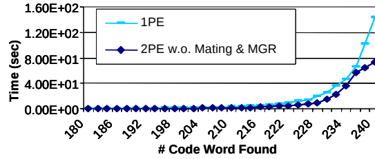
Figure 11 Performance comparison of single PE vs. 2-PE
