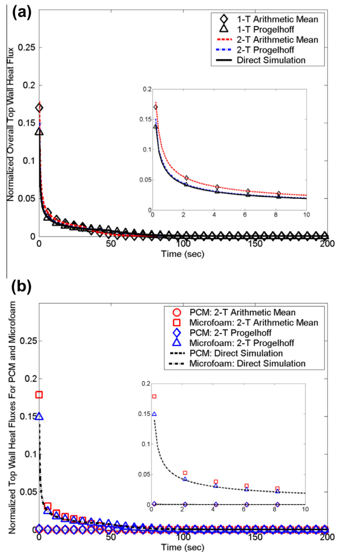
Fig. 7. Heat flux at top surface (a) overall (b) individual component ( T_{top} = 368 K).
