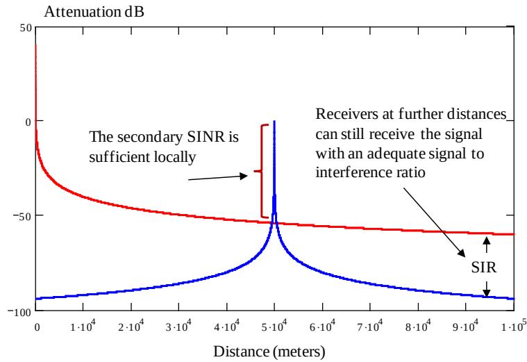
Figure 5-10. A Channel Puncturing Scenario
