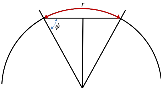
Figure C-4. Effect of Angles on the Occurrence of Occlusion by the Earth's Surface
