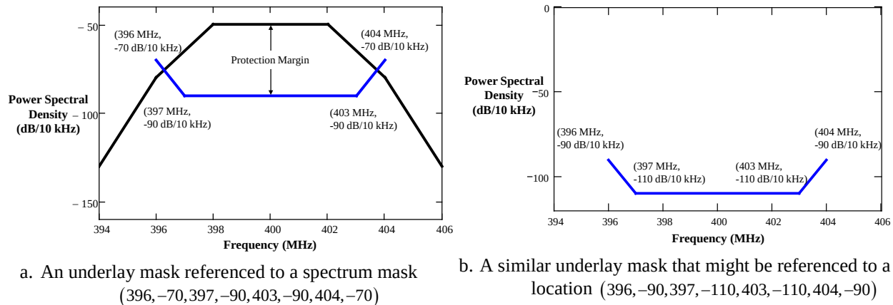
Figure 3-2. Comparison of Underlay Masks with Alternative References
