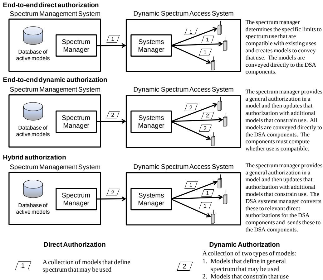
Figure 2-4. DSA Management Methods
