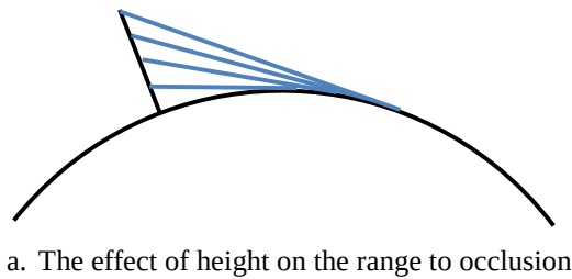
Figure C-4. Effect of Angles on the Occurrence of Occlusion by the Earth's Surface
