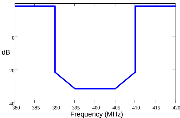
a. Underlay mask of the receiver, 10 kHz RBW
