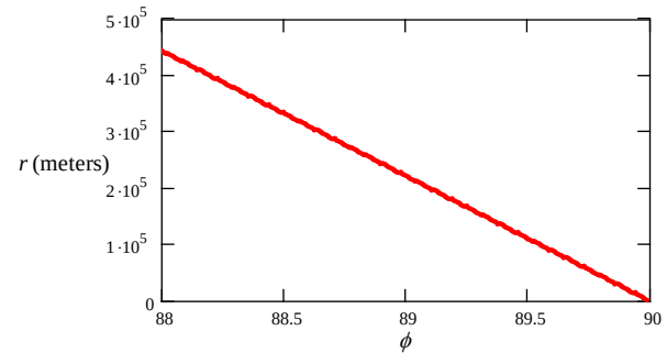
Figure C-4. Effect of Angles on the Occurrence of Occlusion by the Earth's Surface
