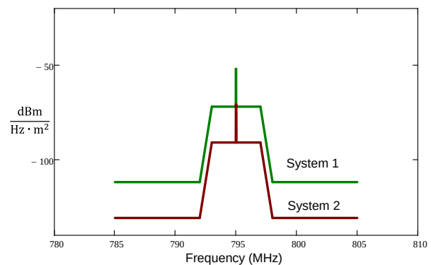
b. Shaped interfering spectrum mask, 10 kHz RBW
