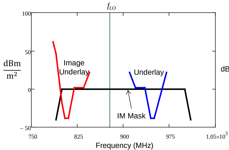
Figure 4-6. Example of Creating an Image Frequency Underlay Mask
