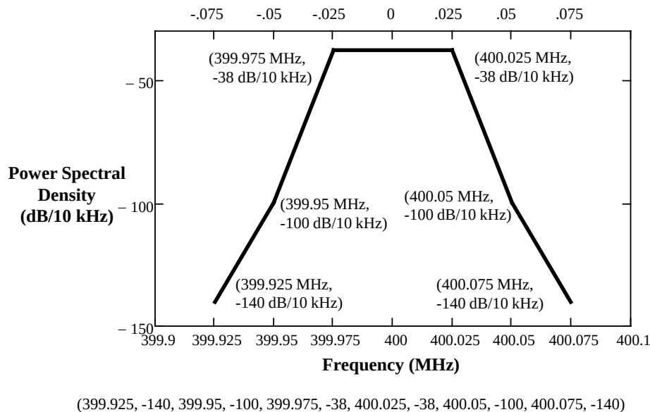
Figure 3-1. Example Spectrum Mask with Its Corresponding Spectrum Mask Vector
