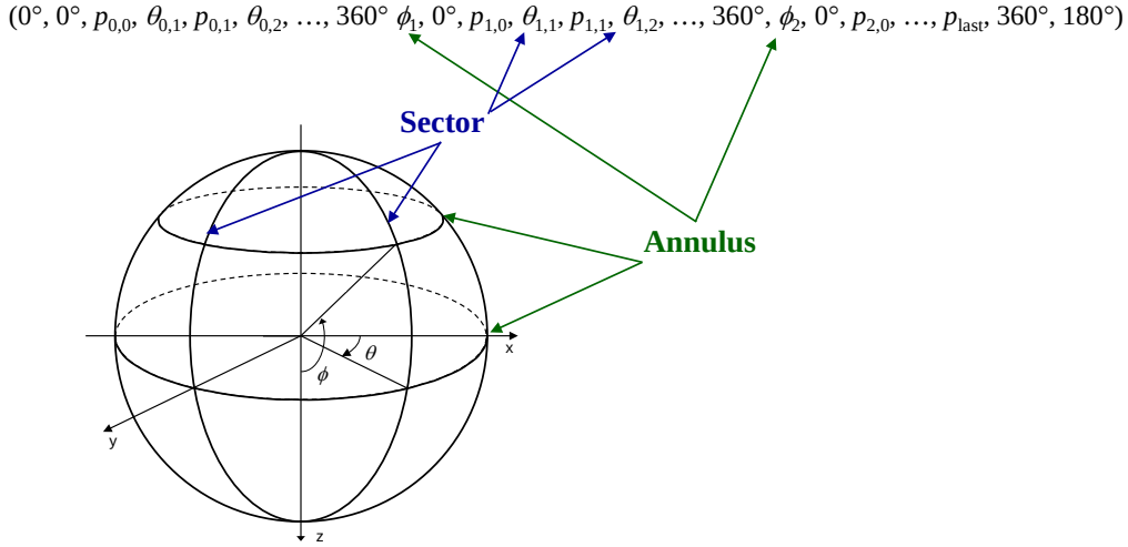
Figure 3-17. Example Map Vector Used in Propagation Map and Power Map Modeling
