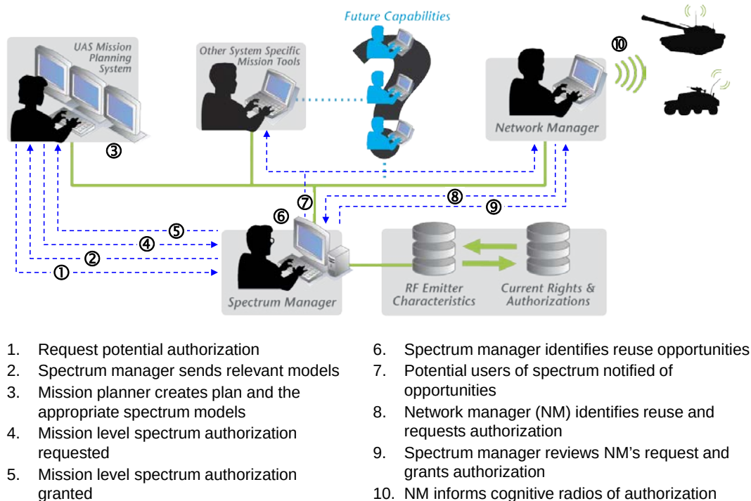
Figure 2-5. Dynamic Spectrum Management Scenario
