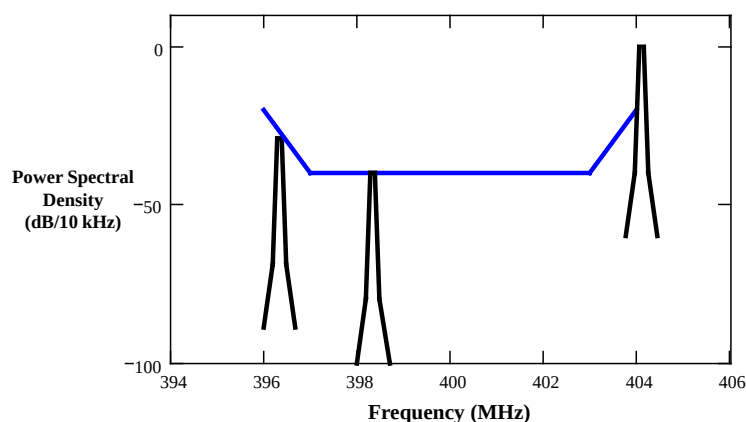
Figure 3-10. Compatible Interfering Signals Using the Maximum Power Spectral Density Method
