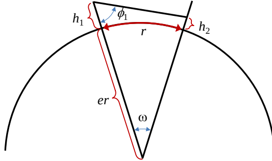
Figure C-7. Geometry of the Spherical Earth Scenario Used to Determine h_2
