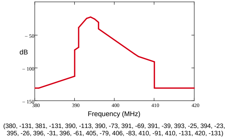
Figure 3-9. The Shaped Spectrum Mask
