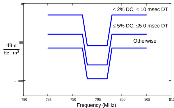
a. Duty cycle rated underlay masks, 10 kHz RBW
