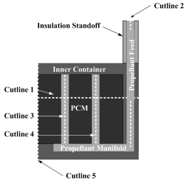
Figure 4: One-half of a cross-sectional view of the equivalent RAC model
