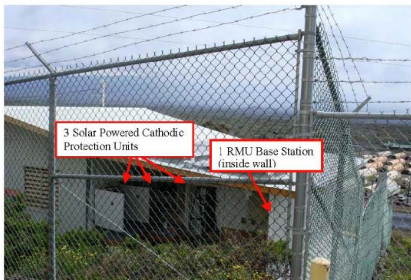
Figure 32: RMU Base Station and location within the building.
