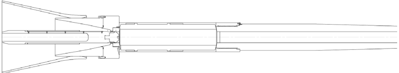
Fig. 4. 105mm RAVEN line drawing .
