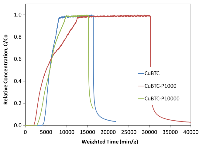
Fig. 4. Ammonia breakthrough results for CuBTC samples. Results show consistent ammonia removal for all three samples.
