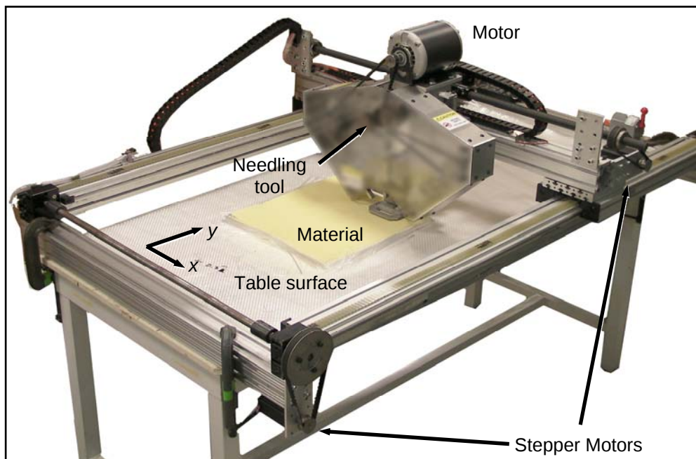
Figure 2. Photograph of the needling facility.
