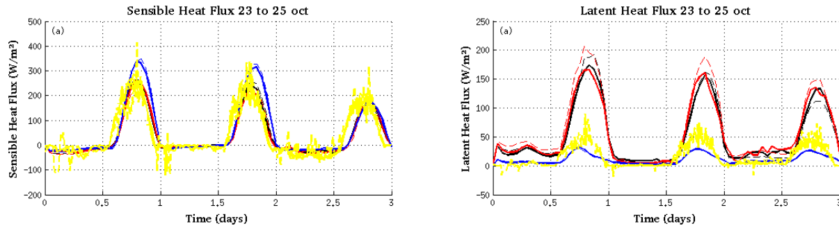
Figure 5. Time series of (left) sensible and (right) latent heat fluxes ( \text{Wm}^{-2} ) in a run where the initial conditions are altered and the soil heat flux is reduced, as discussed in the text (blue) compared to the control run (red and black) and observations (yellow).
