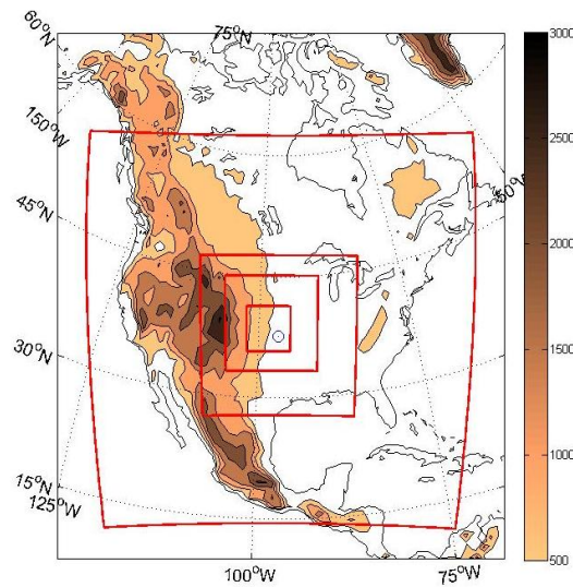
Figure 1 The domain(s) of COAMPS used here showing the outer (parent) domain at 54 km resolution and the three nests at 18, 6 and 2 km resolution, respectively.
