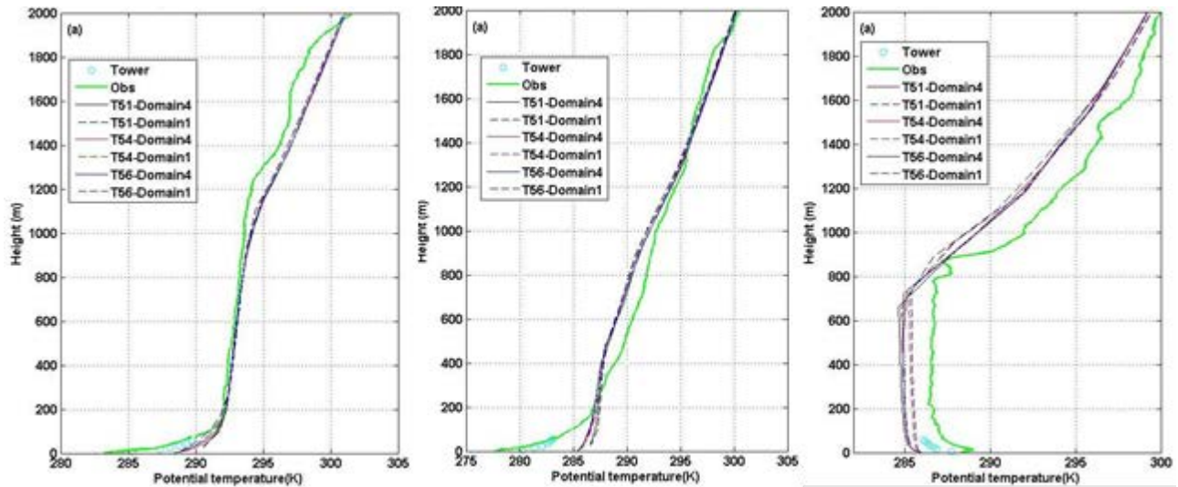
Figure 3. Same as Figure 2 but for potential temperature (K).
