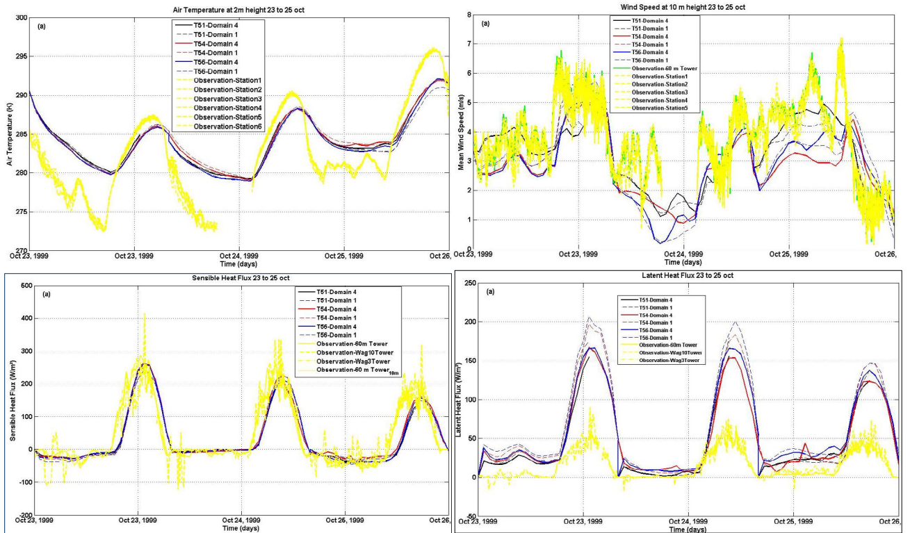
Figure 4. Time series of near-surface variables showing (top left) air temperature (K), (top right) wind speed ( \text{ms}^{-1} ), and of (low left) sensible and (low right) latent heat fluxes ( \text{Wm}^{-2} ).
