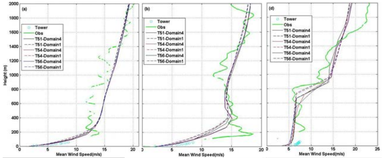
Figure 2. Examples of COAMPS comparison to three soundings for one particular night, 23-24 October, during CASES99. The panels show observed wind speed profiles ( \text{ms}^{-1} , green) from sounding from 22, 04 and 14 local time, left to right. The simulations are from the outmost (Domain 1) and innermost (Domain 4) domains and shows results from two setups, one with 54 model levels with only one within the CASES 50-m mast and one where the near-surface is enhanced by adding two more layers in the lowest 50 m.
