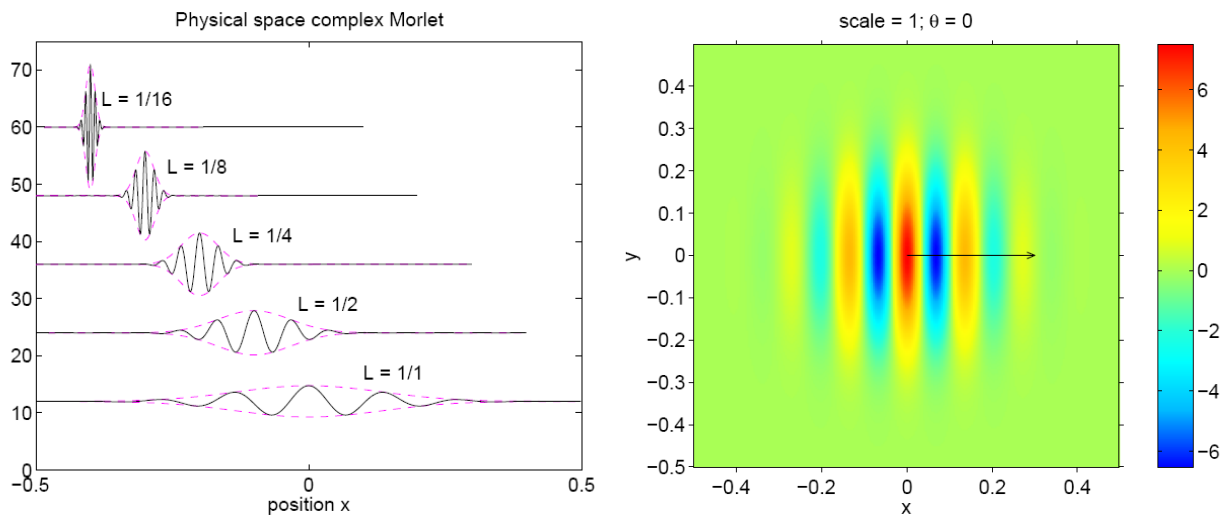
Fig. 1. Morlet wavelet function for 1D space (left) and 2D space (right).
