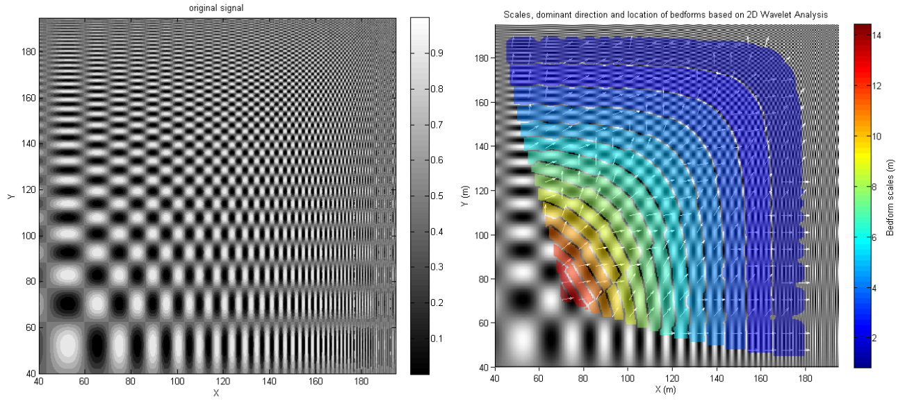
Fig. 3. Results of the 2D WT tool applied to a synthetic bathymetry field with different bedform scales and directions used during the calibration process. Original bed elevation map (left) and identified bedform scales and directions map (right).
