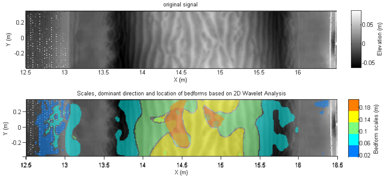
Fig. 4. Results of the 2D WT tool applied to the laboratory bathymetry of Landry (2011) used for validation. Original bed elevation map (top) and identified bedform scales map (bottom).
