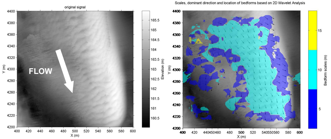
Fig. 6. Results of the 2D WT tool applied to the St. Clair River bathymetry data. Original bed elevation map (left) and identified bedform scales map (right).
