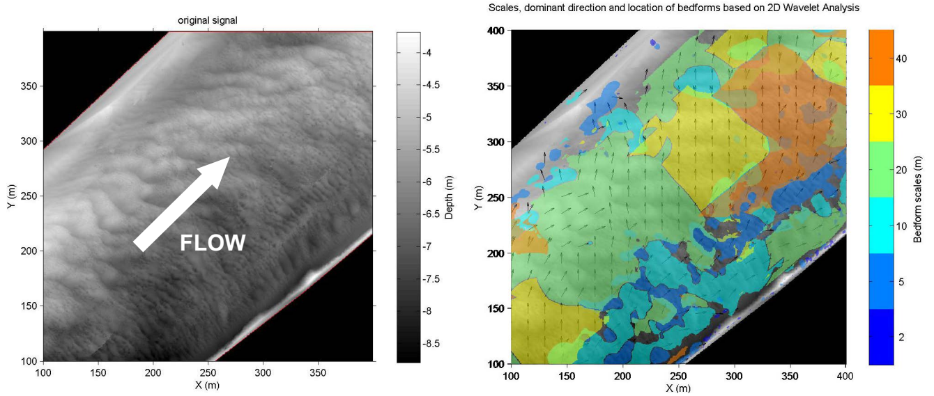
Fig. 5. Results of the 2D WT tool applied to the Missouri River bathymetry data. Original bed elevation map (left) and identified bedform scales map (right).
