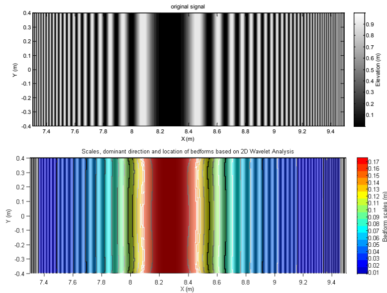
Fig. 2. Results of the 2D WT tool applied to a unidirectional synthetic bathymetry field. Original bed elevation map (top) and identified bedform scales map (bottom).
