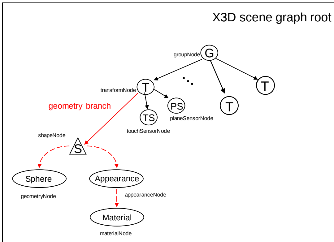
Figure 1. The directed acyclic graph of X3D scene graph objects for the geometry branch of a network node. There is such a description for each of the 26 nodes in the example.
