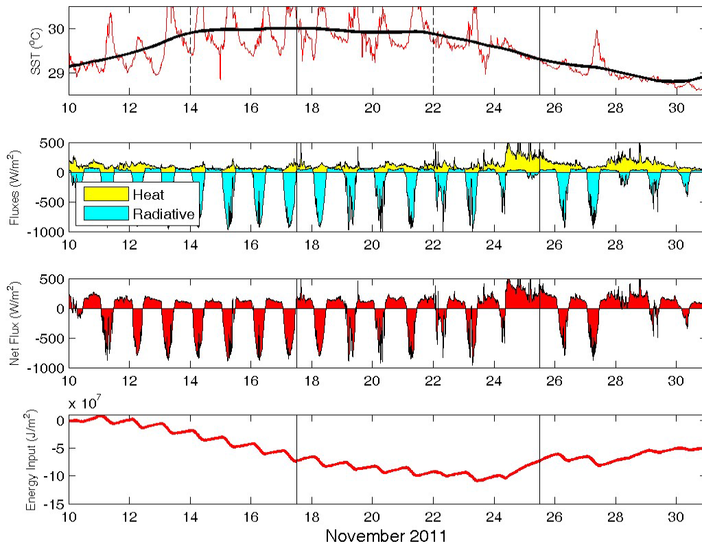
Figure 7. SST (upper panel), heat and radiative flux (2nd panel), net heat flux (3rd panel) and integrated energy flux (lower panel) from data collected during Leg 3.
