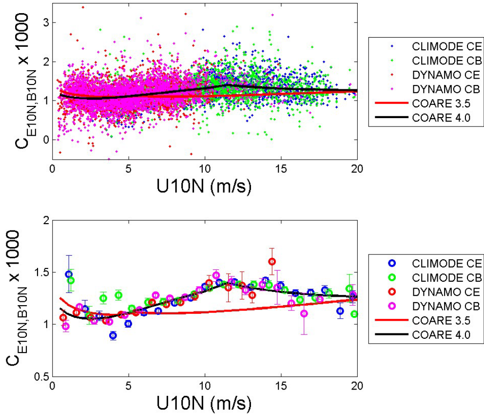
Figure 6. Transfer coefficients for moisture and buoyancy computed from DC fluxes and their associated means. The two sets of transfer coefficients were generated from data collected during DYNAMO/LASP and the CLIMODE programs.
