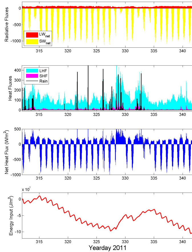
Figure 4. Time series of radiative, surface heat and net heat fluxes during Leg 3. The lower panel shows the integral of the net heat flux over the experiment. A small correction ( \sim 1\% reduction) was applied to the short-wave measurements from the forward mast based on comparison with the PSD and OSU sensors. A more significant correction to the long-wave measurements was applied to the mast using the PSD sensors. The latent, sensible and rain induced fluxes are computed using COARE 3.5.
