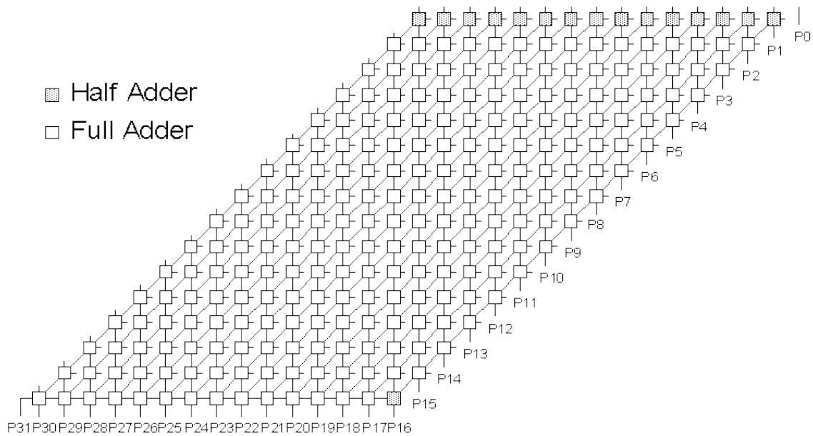
Figure 13: ISCAS-85 C6288 circuit [11].
