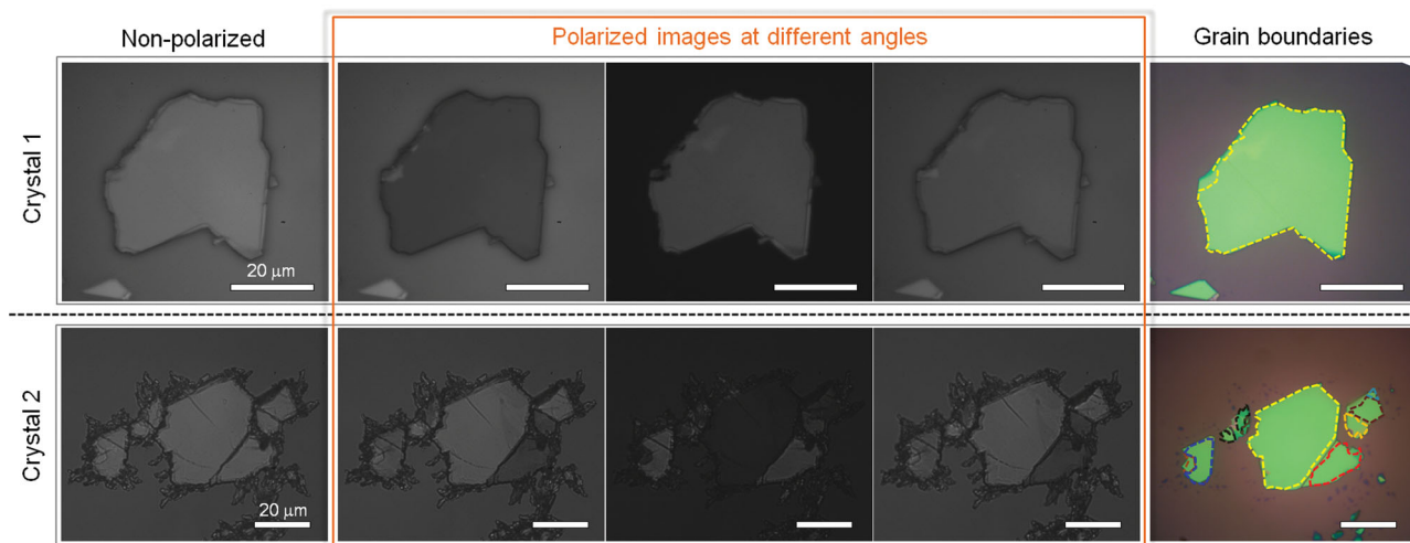
Figure 3. Rubrene crystalline films with large single-crystalline domains grown on h-BN. Polarization optical characterization for two representative samples. The normal (1st column) and polarized (2nd–4th columns) images at different angles are shown for each samples. The last column shows the grain map overlapped on the optical image of h-BN flakes. Crystal grains and grain boundaries are distinguished clearly by an optical contrast in polarized images and indicated by dashed lines with different colors in maps.
