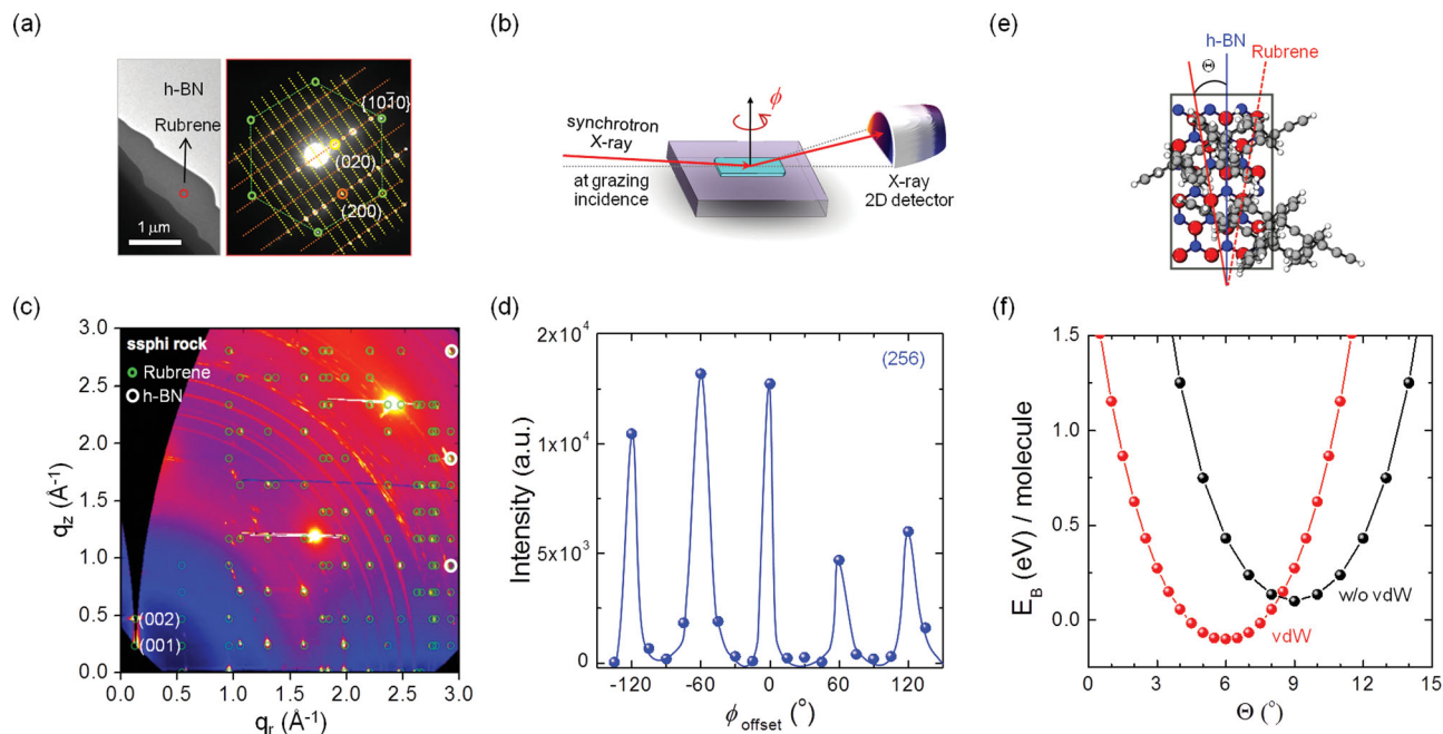
Figure 2. VdW epitaxial relation between rubrene and h-BN crystals. a) Bright-field TEM image and selected-area electron diffraction pattern of the rubrene crystal grown on h-BN. The rubrene (200), (020) and h-BN {10 \bar{1} 0} planes are indicated by orange, yellow and green circles, respectively. b) Schematic of GIXD measurements. c) Measured and calculated 2D GIXD patterns of rubrene crystals grown on h-BN. Green and white circles represent the calculated diffraction patterns for orthorhombic rubrene and h-BN crystals, respectively. The two dominant bright features observed at the diffraction point, ( q_x, q_z ) \approx (2.4 Å -1 , 2.5 Å -1 ) and \approx (1.2 Å -1 , 1.7 Å -1 ) originate from the Si substrate underneath the thermally grown SiO 2 layer. d) Representative azimuthal ( \phi )-scan of GIXD for the (256) plane of rubrene, which shows the regular diffraction peaks with 6-fold symmetry. e) Top-view image of rubrene molecules on the h-BN surface using a ball-stick model. The black box defines the supercell used in the calculations with the definition of the in-plane misorientation angle ( \Theta ). f) Plot of the binding energy per rubrene molecule as a function of \Theta obtained from first-principles calculations. The red and black curves represent the calculations with and without vdW interactions, respectively.
