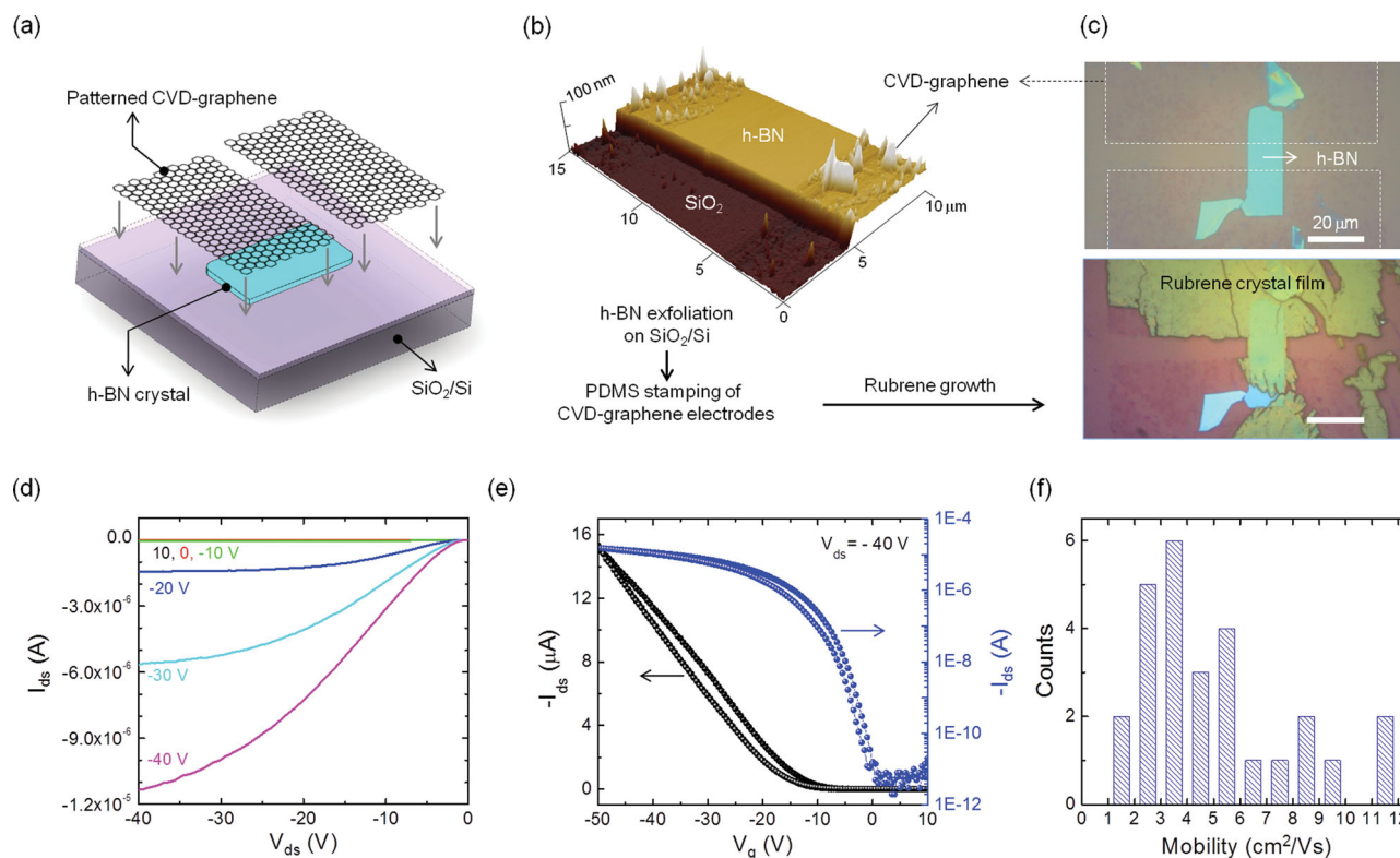
Figure 4. Fabrication and electrical characterization of FETs using graphene electrodes. a) Schematic illustration for the fabrication of graphene electrodes on h-BN. b) AFM image of the patterned CVD-graphene electrodes on the h-BN/SiO 2 substrate. c) Optical images of the device before (top) and after (bottom) rubrene crystal growth on the stacked graphene/h-BN structure. d,e) Representative output (d) and transfer (e) characteristic curves of FETs with graphene electrodes. f) Histogram of mobility measured from 27 devices. The average and maximum values of mobility are 5.1 \pm 2.7 \text{cm}^2 \text{V}^{-1} \text{s}^{-1} and 11.5 \text{cm}^2 \text{V}^{-1} \text{s}^{-1} , respectively.
