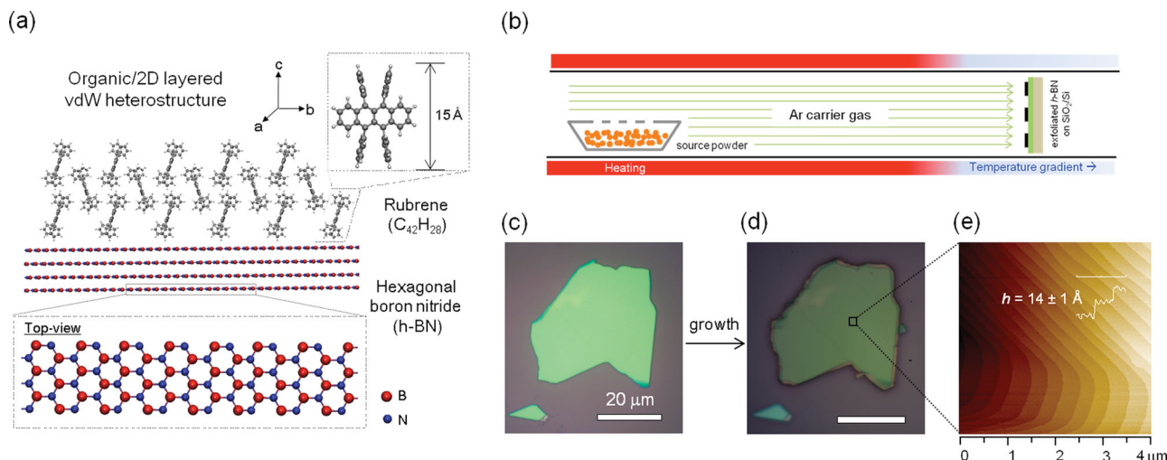
Figure 1. Growth of organic/2D layered vdW heterostructures. Schematic illustration of: a) the organic/2D layered vdW heterostructure composed of rubrene and h-BN and b) the vapor-phase transport method for the growth. Optical images of: c) the h-BN crystal exfoliated on a SiO 2 /Si substrate and d) the rubrene film grown on h-BN. e) AFM image of the film surface and the height profile along the line. It shows a highly uniform terrace structure with the step height of 14 \pm 1 Å.
