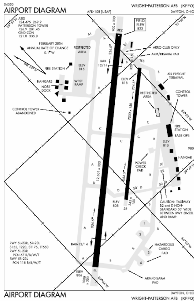
Figure 3-2. Wright-Patterson AFB Airfield Diagram
