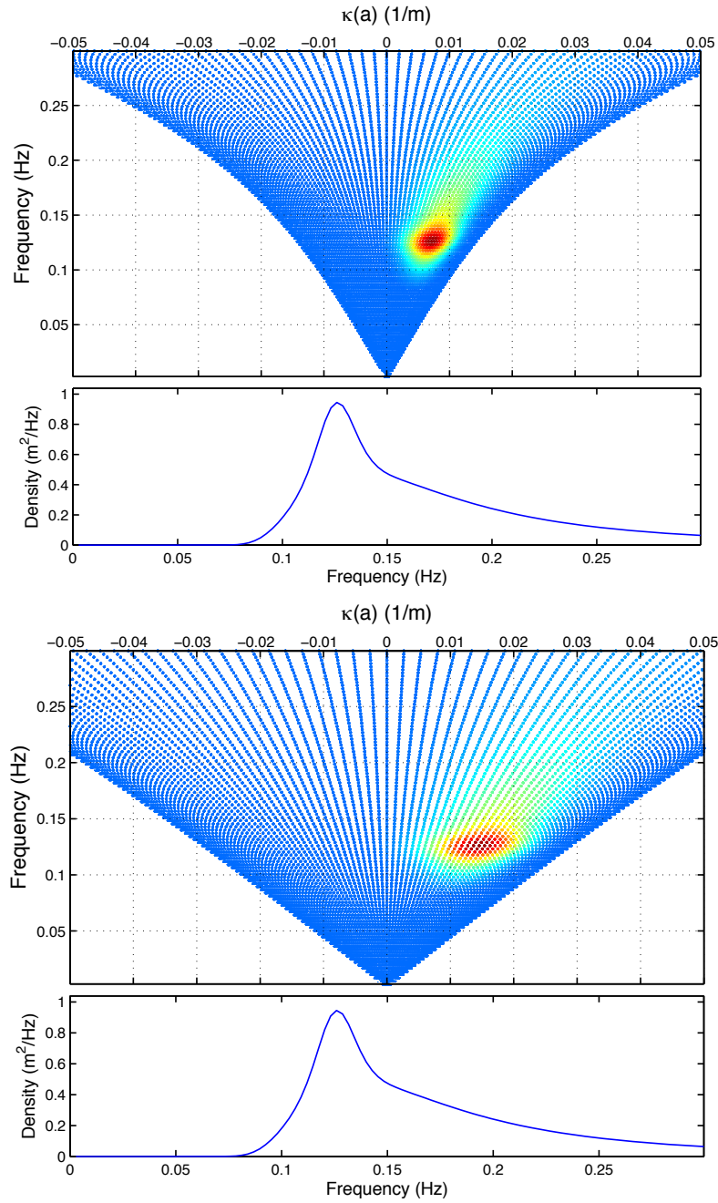
Figure 3. Output from the nonlinear directional wave model. Top: Initial condition – directional spectrum at h=10\text{m} remapped into (f, \kappa) space. Bottom: Model output at h=2\text{m} .
