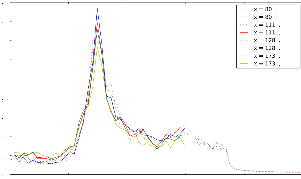
Figure 2. Comparison of spectra from parabolic nonlinear wave model (solid line) to data from Louisiana shelf experiment (dotted line). Input waves were oriented 30 degrees to shore normal; comparisons to data here are more favorable than those oriented normal to shore.
