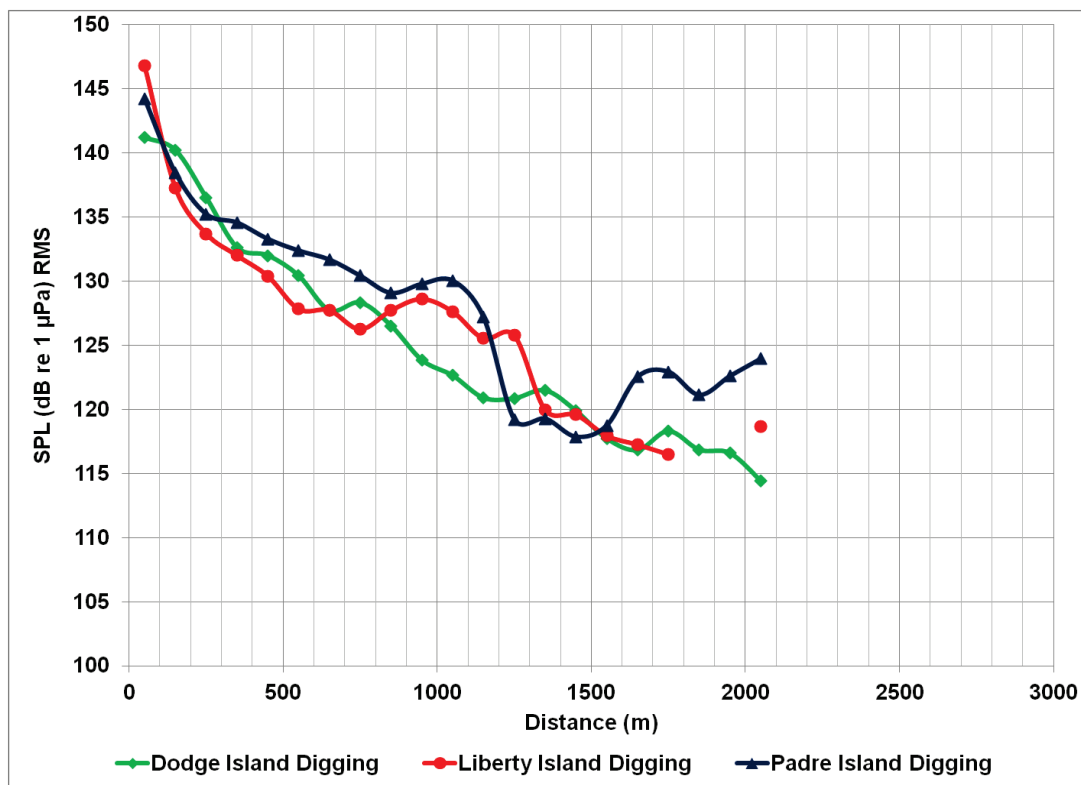
Figure 5. Comparison of SPL (dB rms) during sediment excavation.
