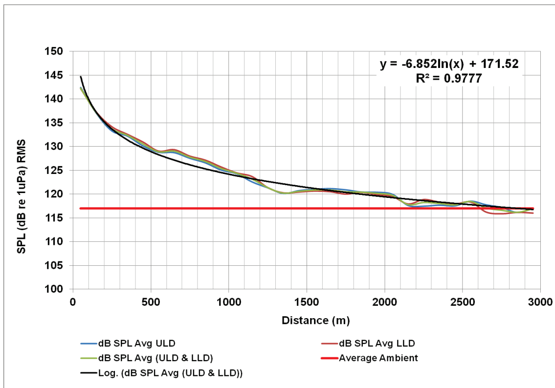
Figure 18. SPL (dB re 1 \mu Pa RMS) versus distance for all dredges and dredging events combined.
