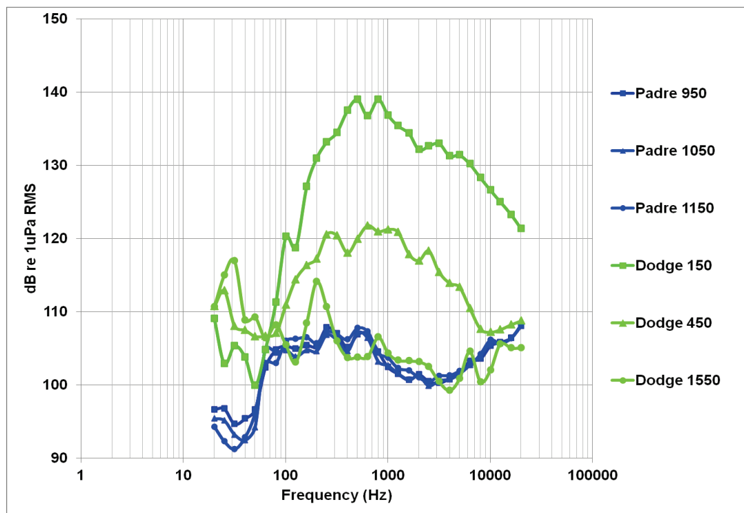
Figure 14. Results (1/3-octave) at selected distances during transition from transit to digging.
