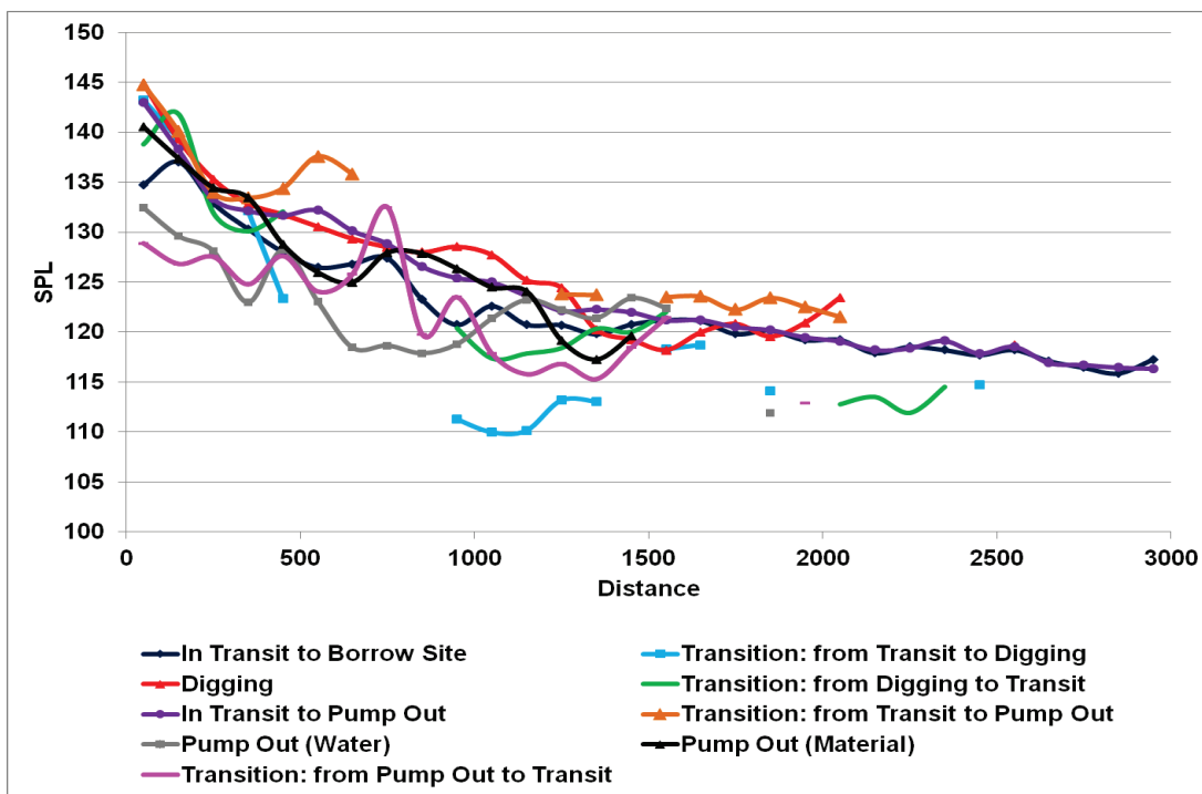
Figure 17. SPL (dB rms) versus distance by dredging activity. SPLs logarithmically averaged by activity for all three dredges.
