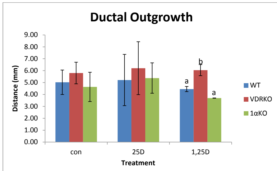
Figure 13. Ductal outgrowth analysis of WT, VDRKO and 1 \alpha KO mammary glands grown in culture and treated with 500nM 25D, 100nM 1,25D or ethanol control. Treatment of glands with the active metabolite of vitamin D, 1,25D elicited a difference in the extension of the ductal branching network into the mammary fat pad between the VDRKO model and the 1 \alpha KO and WT models ( p=0.001 ). (letters indicate statistical difference to the WT group for that treatment calculated by ANOVA)
