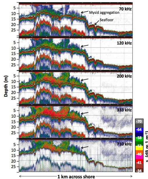
Figure 3. Acoustic backscatter from shipboard echosounders at five-frequencies show the highly aggregated distribution of mysids and the abrupt end of these aggregations at water depths of around 20 m. The frequency response can be used to estimate the size class of mysids throughout the aggregation.
