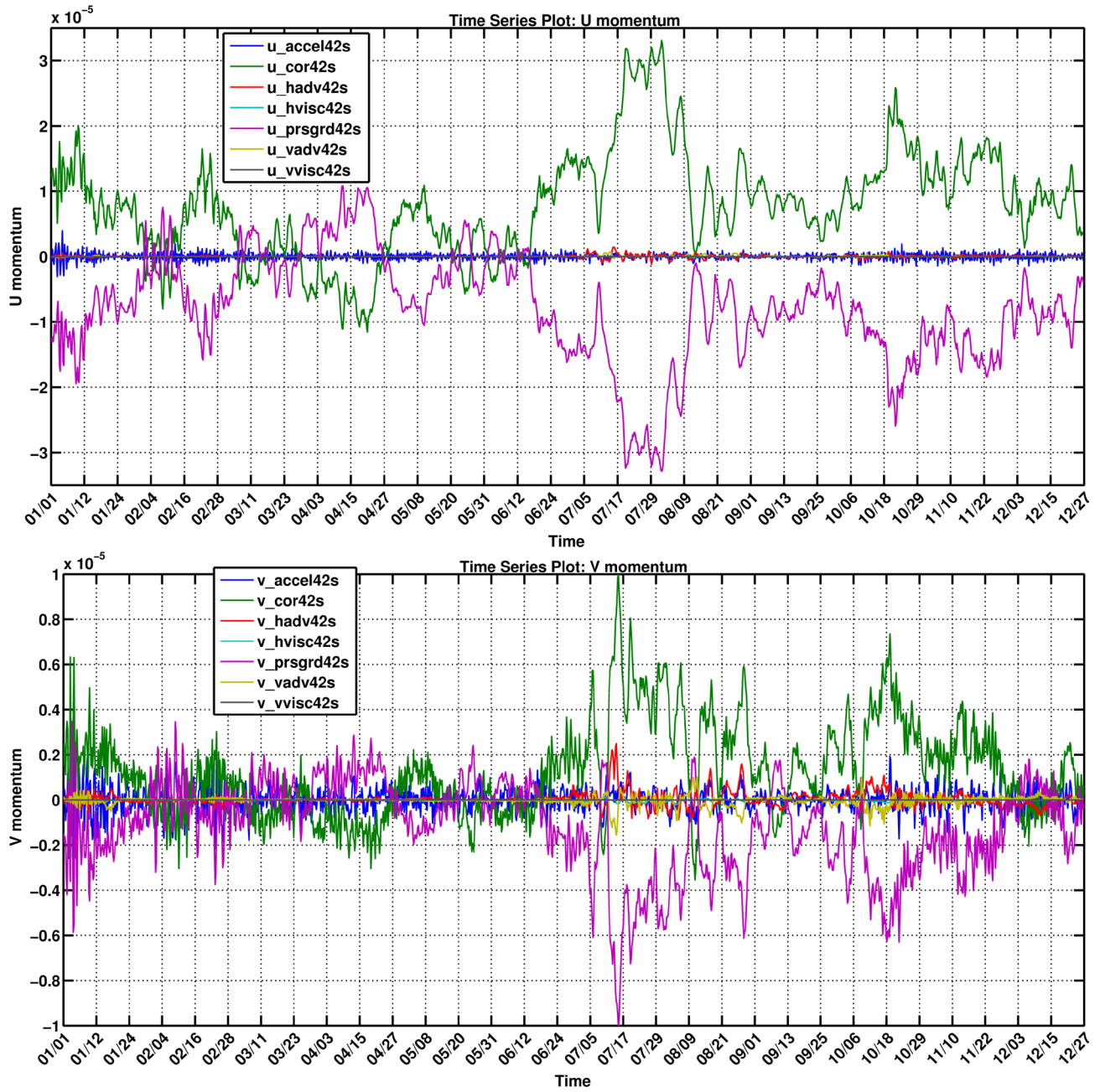
Figure 1. Time series of zonal (top) and meridional (bottom) momentum balance for a point within the undercurrent ( -124.76^{\circ}W, 42^{\circ}N, -250m ) vs. month/day for year 2005. Both balances are geostrophic to first order. The meridional balance shows significant departures from geostrophic balance, with contributions from horizontal advection (red) and local acceleration (blue).
