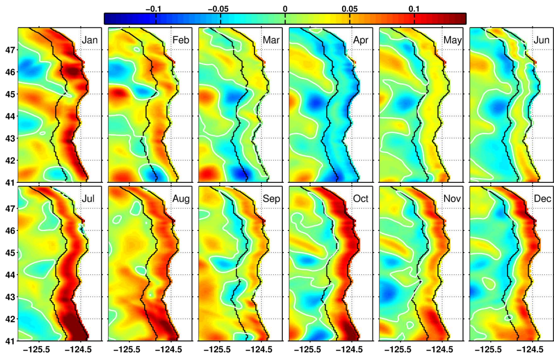
Figure 3. Monthly Eulerian-mean meridional velocity ( \text{m s}^{-1} ), averaged over the depth range 150 - 500 m (or the bottom, in depths less than 500 m). The zero contour is indicated (white). The 200-m isobath and the longitude points 36 km west of the 200-m isobath (approximately the 850-m isobath) are indicated (black contours). In white is the zero-velocity contour.
