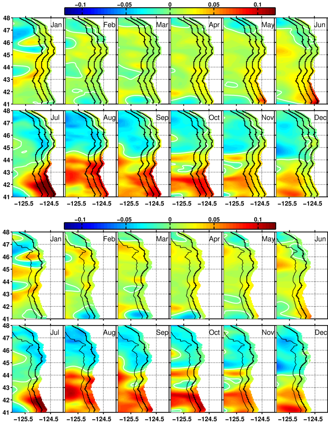
Figure 2. Monthly-mean depth-averaged dynamic height anomaly (m) for depths 150-500 m (upper panels) and 500-1250 m (lower panels) vs. longitude and latitude. The zero contour is indicated (white). The 200-m isobath and the longitude points 36 km west of the 200-m isobath (approximately the 850-m isobath) are also indicated (outer black contours), along with the points midway between these at constant latitude (central black contour).
