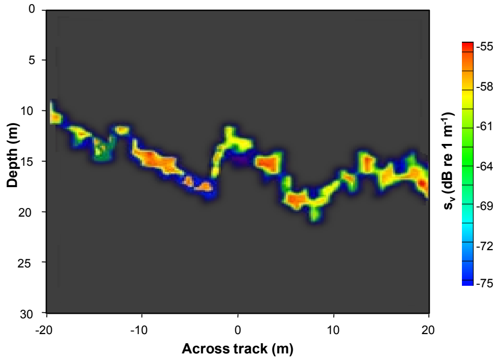
Figure 1. The top panel shows an example transect of acoustic scattering at 120 kHz. The bottom panel shows the regions identified as containing an acoustic thin layer in red.
