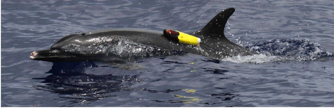
Figure 1. Photograph of the Acousonde™ 3B hydrodynamic acoustic recording tag attached with suction cups to a pantropical spotted dolphin (photo by Robin Baird, Cascadia Research, NMFS Scientific Research Permit No. 731-1774)
