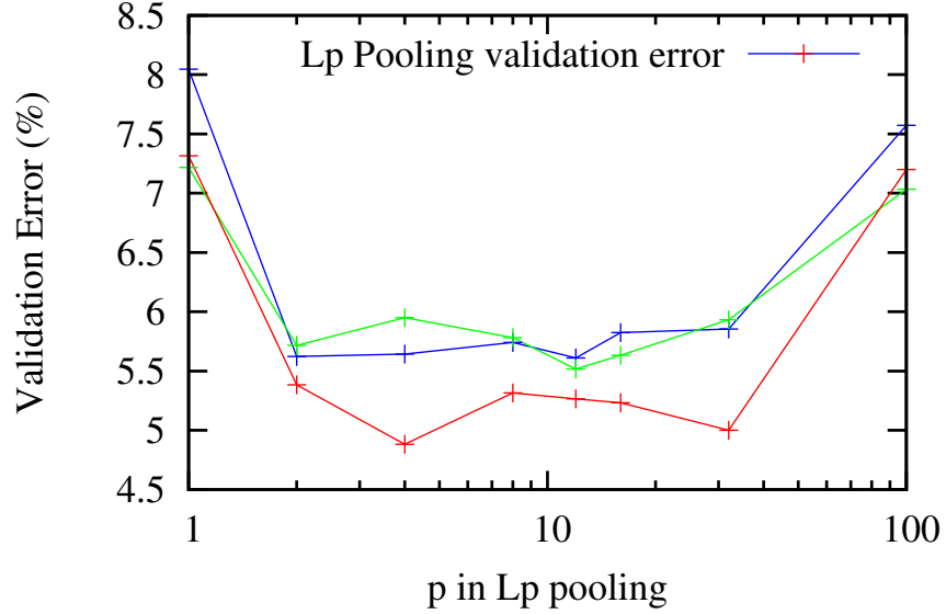
Figure 3.10: Error rate of Lp-pooling on 3 cross-validation sets for p = 1, 2, 4, 8, 12, 16, 32, \infty ( p = \infty is represented as p = 100 for convenience). These validation errors are reported after 1000 training epochs.
