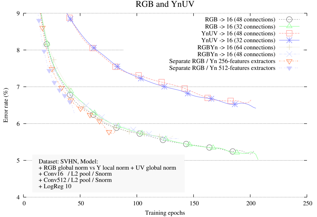
Figure 3.12: Comparison of house numbers classification performance with (YnUV) and without preprocessing (RGB). Regardless of the connection scheme to the input channels, the non-preprocessed data (RGB) improves by 1 point over the preprocessed data.
