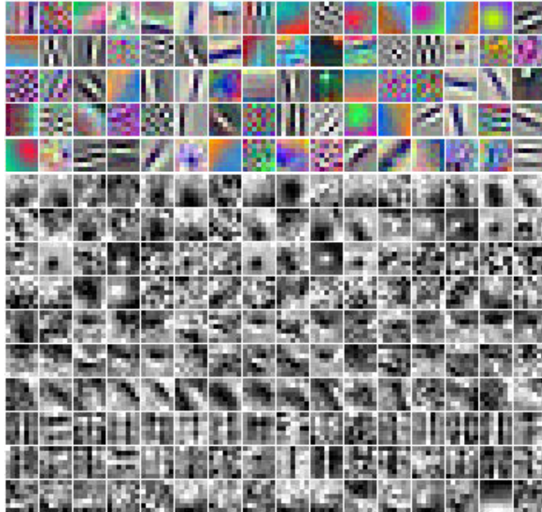
Figure 3.3: Layer 1 (top) and layer 2 filters (bottom).
