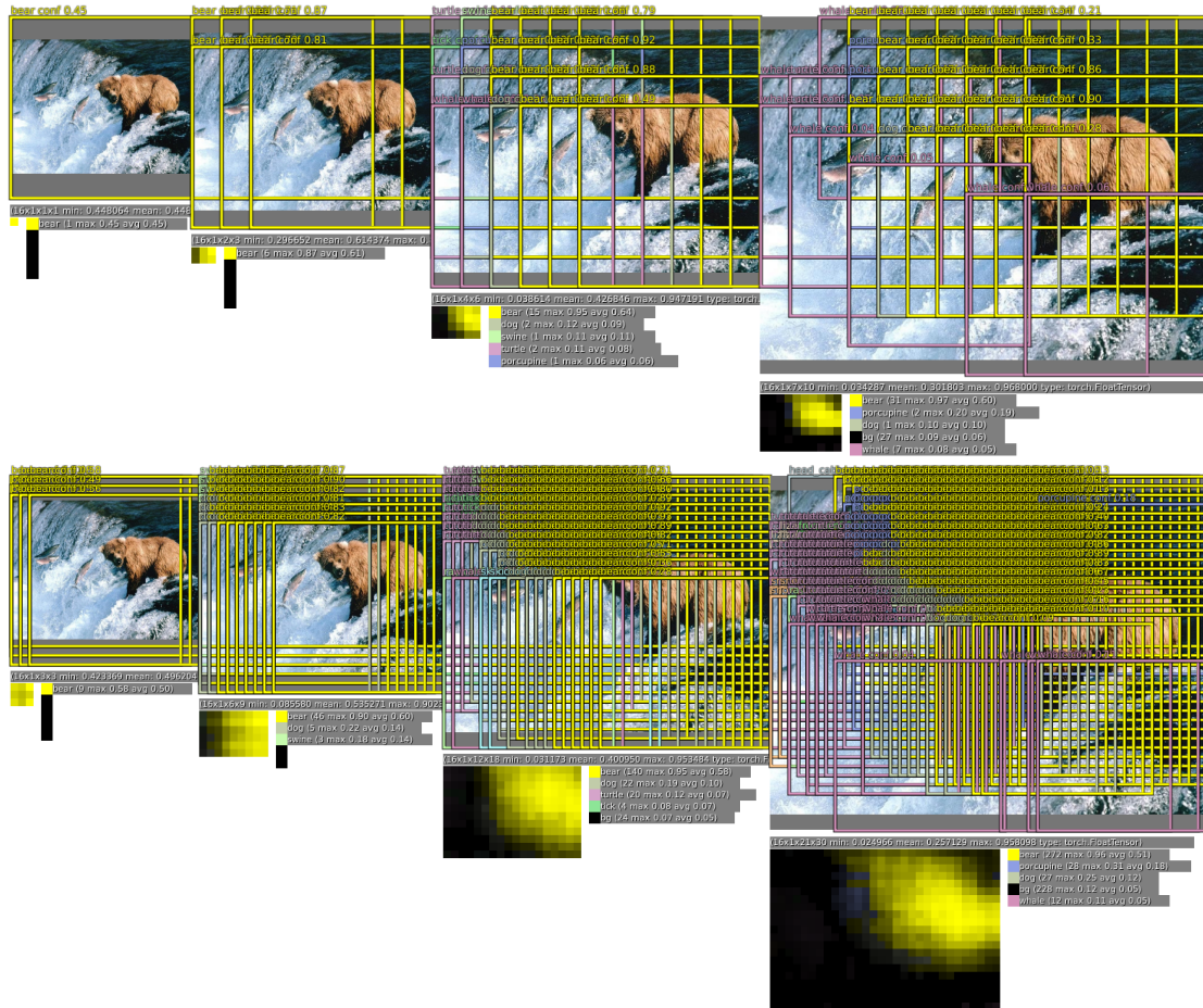
Figure 4.8: Localization/Detection pipeline: fine stride sliding window. The raw classifier/detector outputs a class and a confidence for each location (top). The resolution of these predictions can be increased using the method described in section 3.1.3 (bottom).
