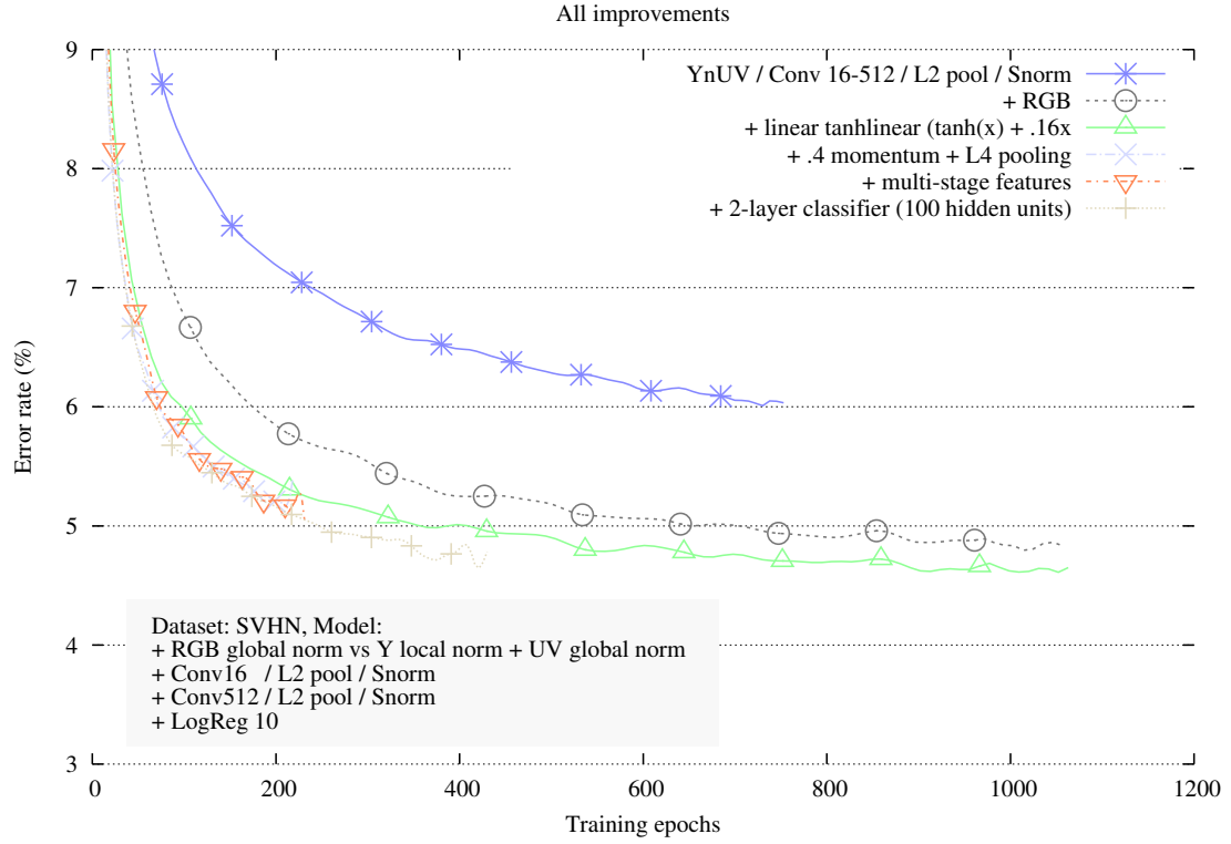
Figure 3.17: A summary of architecture improvements over [17]. From top to bottom we incrementally add architectural changes to the baseline model published in [17]. The biggest error rate decrease is induced by changing the normalized YUV input to an un-normalized RGB input, followed by the use of a twisted tanh over a regular tanh sigmoid nonlinearity. Minor improvements are then added with an intermediate momentum, L4 pooling instead of L2, multi-stage features and a 2-layer classifier.
