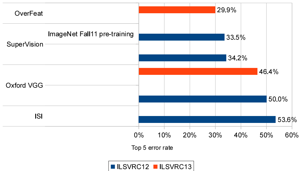
Figure 4.14: ILSVRC12 and ILSVRC13 competitions results (test set). Our entry is the winner of the ILSVRC13 localization competition with 29.9% error (top 5). Note that training and testing data is the same for both years. The OverFeat entry uses 4 scales and a single-class regression approach.
