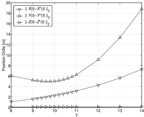
Fig. 9 \ell_2 -norm of position errors as functions of control gain 8 \leq \gamma \leq 14 .
