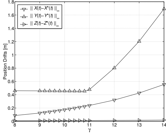
Fig. 7 \ell_\infty -norm of position errors as functions of control gain 8 \leq \gamma \leq 14 .
