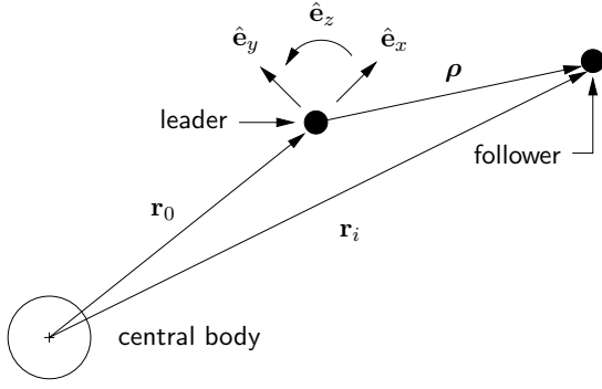
Fig. 1 Leader-follower geometry with \hat{e}_x \times \hat{e}_y = \hat{e}_z .
