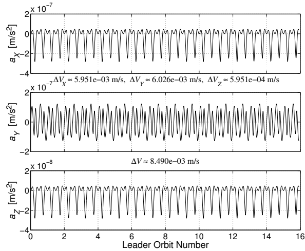
Fig. 13 Control accelerations and \Delta V 's using linear constraint manifold with \gamma^* .
