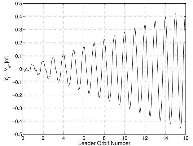
Fig. 11 Along-track position difference between the linear and controlled nonlinear solution with \gamma^* .
