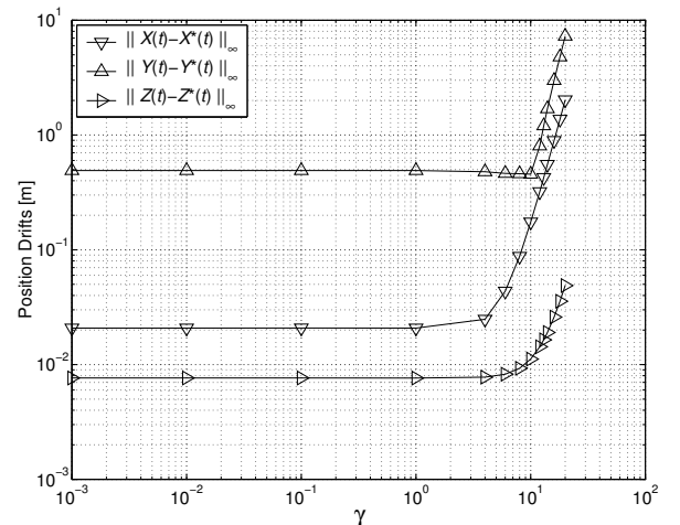
Fig. 6 \ell_\infty -norm of position errors as functions of control gain \gamma .
