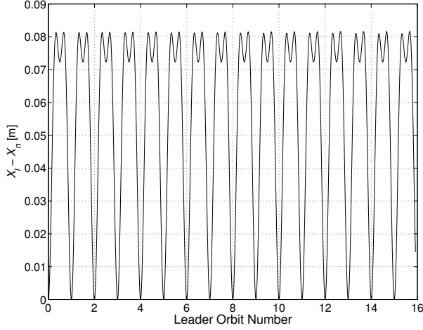
Fig. 3 Radial position difference between the linear and nonlinear Hill's equations.
