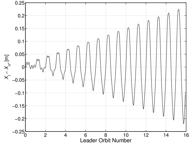
Fig. 10 Radial position difference between the linear and controlled nonlinear solution with \gamma^* .
