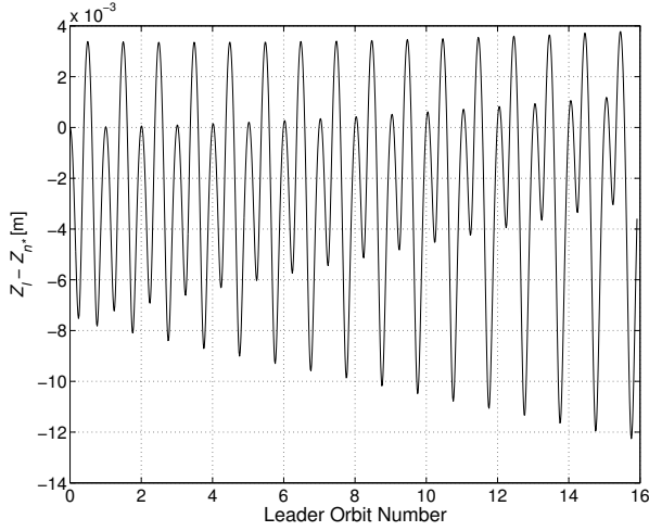
Fig. 12 Cross-track position difference between the linear and controlled nonlinear solution with \gamma^* .
