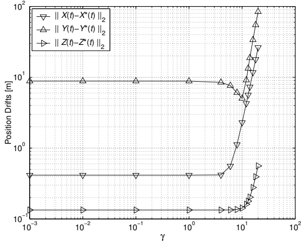
Fig. 8 \ell_2 -norm of position errors as functions of control gain \gamma .
