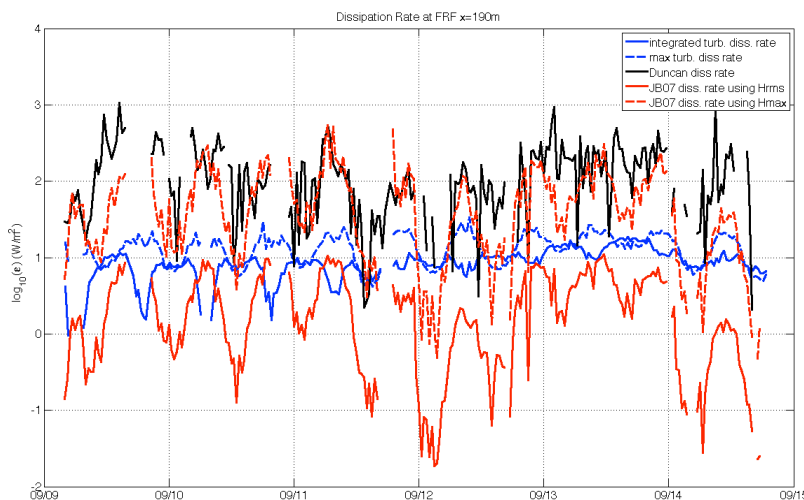
Figure A4. In situ TKE dissipation rates (provided by Jim Thomson) compared against IR-derived wave dissipation rates at location near the bar crest, x = 190\text{m} . Tidal modulation in dissipation is evident in all the estimates and the in situ estimates are approximate 1-1.5 orders of magnitude lower than the IR-based estimates.
