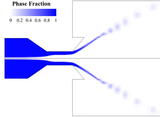
Figure 8. Instantaneous phase contour of atomizer internal flow
