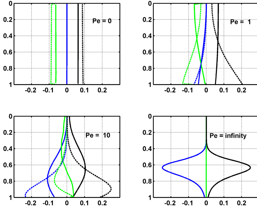
Figure 3 Steady state ( t \rightarrow \infty, \frac{\partial \bar{P}}{\partial t} = 0 ) contribution of the terms of equation (28)- advection, term II, blue lines; turbulent diffusion, term III, green lines; and the growth rate (reaction), R , term IV, black lines. As in figure 1, the solid lines refer to Case A, the dashed lines, Case B. Note that: the advection term II, blue line, is always negative and indicates an upward flux of material; the turbulent diffusion term, III, green line, can be either sign with negative a downward flux of material and positive an upward flux; the reaction (growth rate) term, III, black line, is always positive. The three terms must balance in the steady state. Four cases, each of different Peclet number, Pe , are shown.
