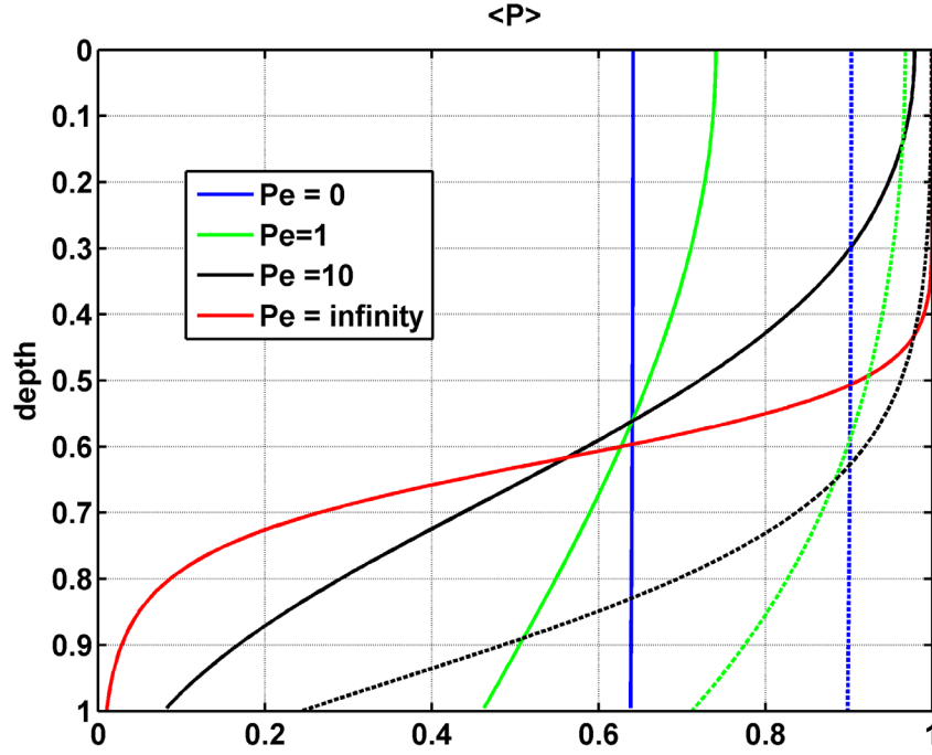
Figure 2 Steady state ( t \rightarrow \infty, \frac{\partial \bar{P}}{\partial t} = 0 ) vertical profiles of \langle P \rangle for the Peclet number, Pe , indicated in the figure, using \alpha = 1 . . Case A, the solid color coded lines are the solutions for \langle P \rangle obtained by using (27a) with (26b) as the PDF, TIBI term included. Case B, the dashed color coded lines, the solution to the ADR equation (28) with the TIBI term neglected, R = R_0 .
