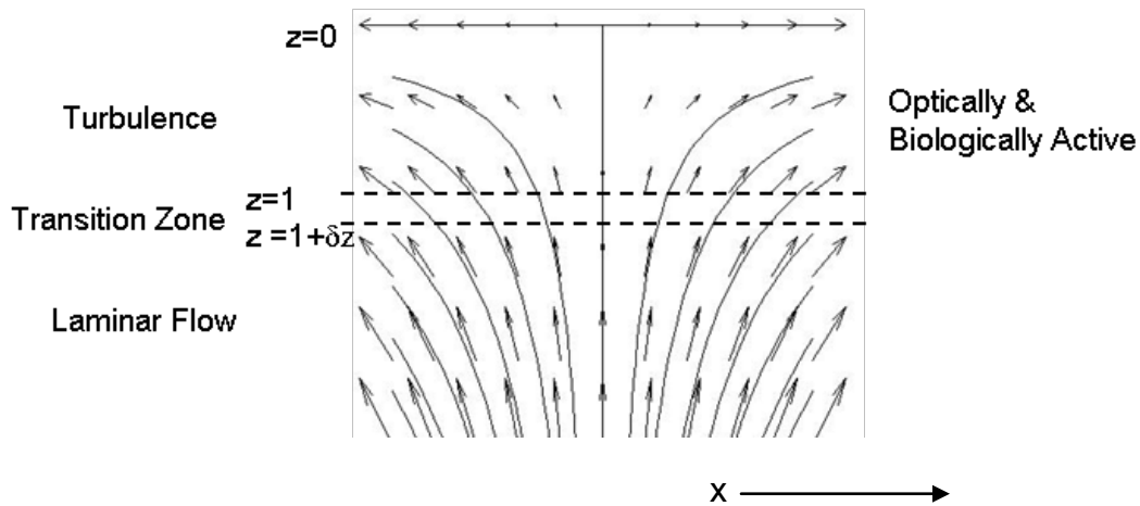
Figure 1. Upwelling flow field into an optically and biologically active mixed layer used in the Goodman and Robinson (2007) biodynamical model. Note as \alpha increases or as the uptake time increases relative to the advection time
